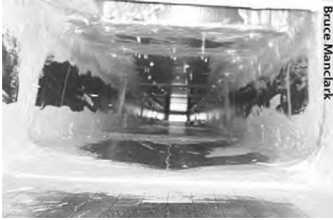
Lining a panned cavity: Foil-faced foam board, designed for lining cavities is sealed with duct mastic to provide an airtight return.
