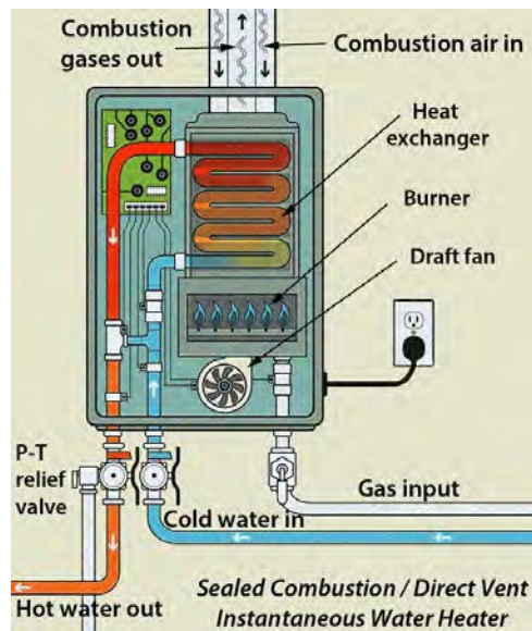
Sealed-combustion tankless water heater: These water heaters have a small market share and save around one-third of energy used by the best storage water heaters.
