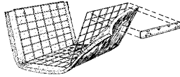
Washable filter installed on a rack inside the blower compartment.
