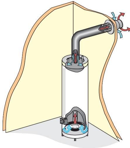
Direct-vent water heater: Moves combustion air and flue gases through a concentric pipe system without a draft fan.
