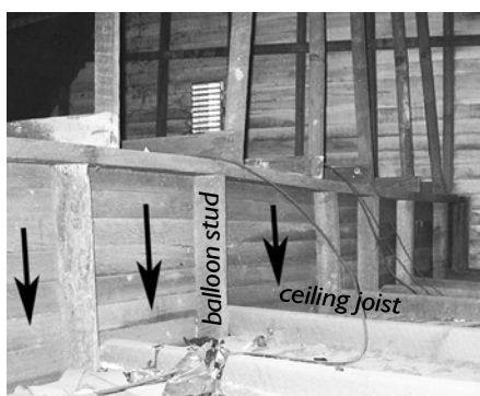
Balloon framed walls: Wall cavities, shown from outdoors at right and from the attic at left, are open to the floor cavity, the attic, and the crawl space.
