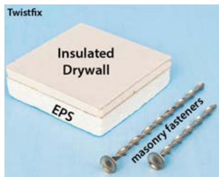
Insulated drywall: This specialty product works well for masonry and plaster interior walls.
