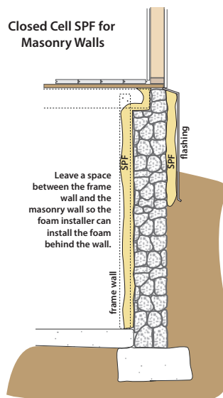
2-part foam sprayed on rubble masonry: Installers insulate rubble masonry walls on the interior or exterior with sprayed plastic foam. On the interior, they cover the foam with drywall.
