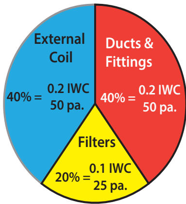
Typical static pressures in IWC, pa, and percent of total static pressures for a typical well-designed and installed split-system air conditioner.
