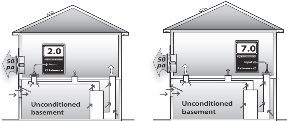
Pressure pan test: A pressure pan reading of 2 indicates moderate duct air leakage in the supply ducts.
