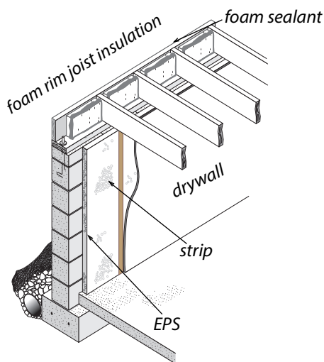
2-inch foam board with plywood strips: Installers fasten foam to the foundation wall using built-in strips. They then attach the drywall to the strips in the foam.
