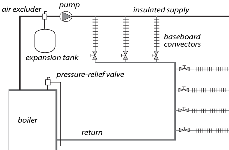
Simple reverse-return hot-water system: The reverse-return method of piping is the simplest way of balancing flow among the heat emitters.
