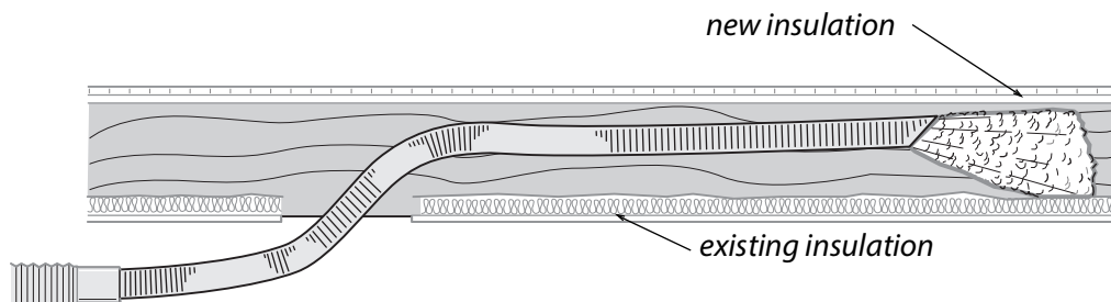
Blowing bellies: A flexible fill-tube, which is significantly stiffer than the blower hose, blows fiberglass insulation through a hole in the belly from underneath the home.
