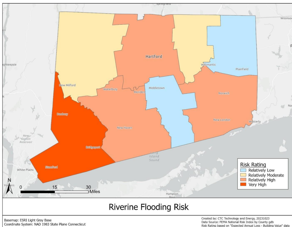
Figure 4: Riverine Flooding Risk in Connecticut
