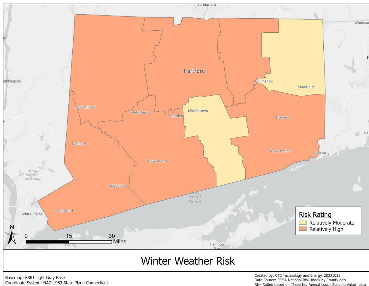
Figure 10: Winter Weather Risk in Connecticut
