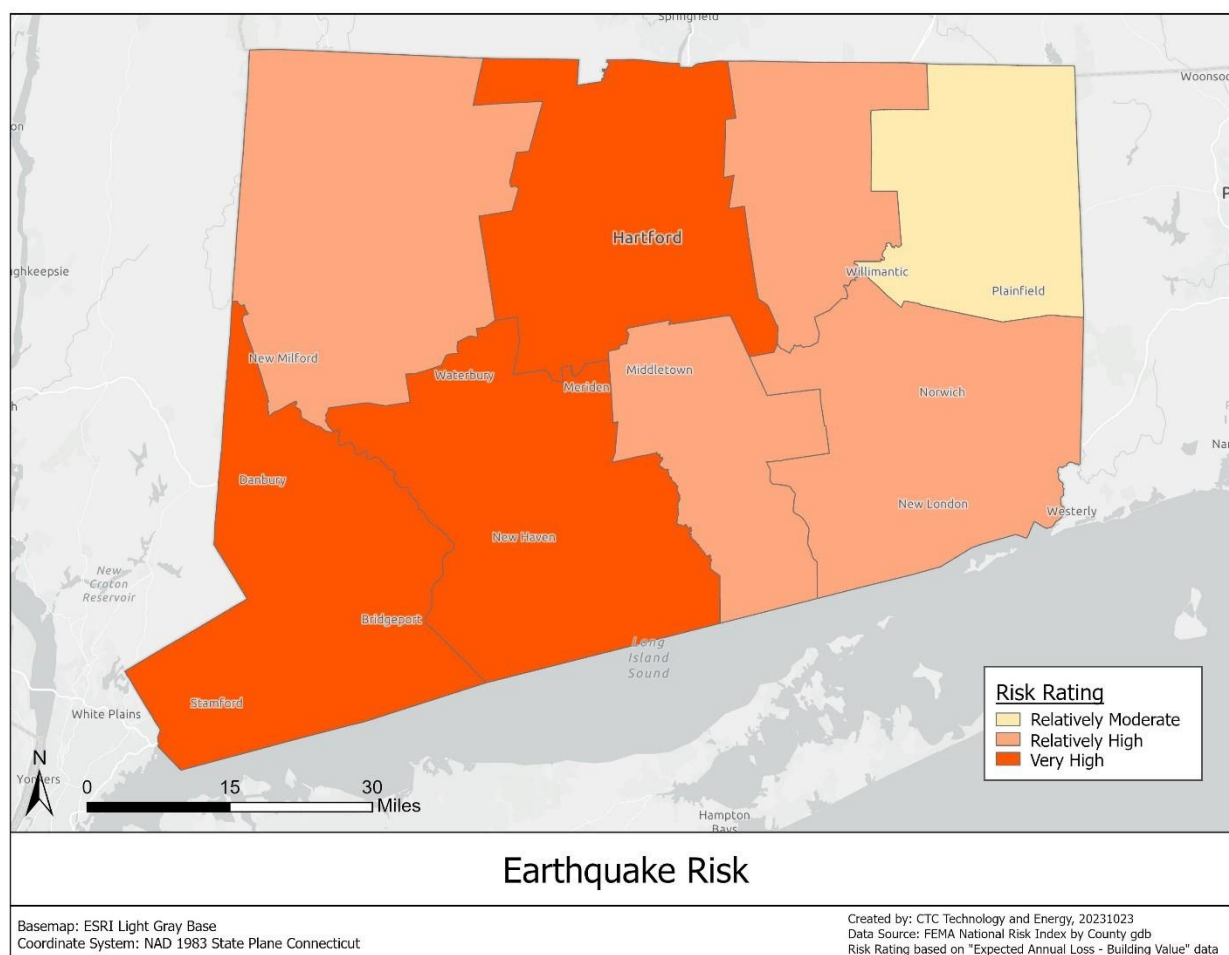
Figure 14: Earthquake Risk in Connecticut
