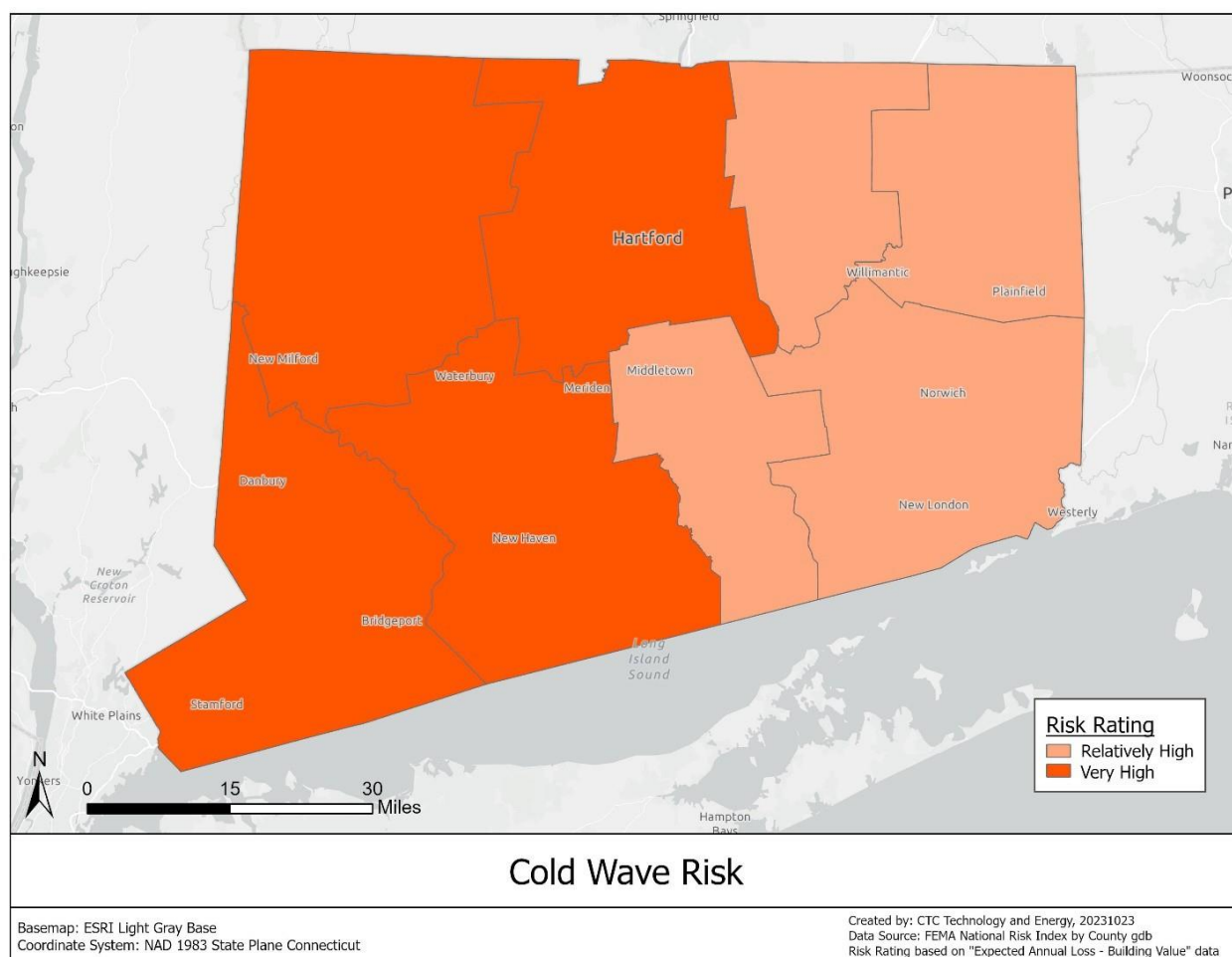
Figure 11: Cold Wave Risk in Connecticut
