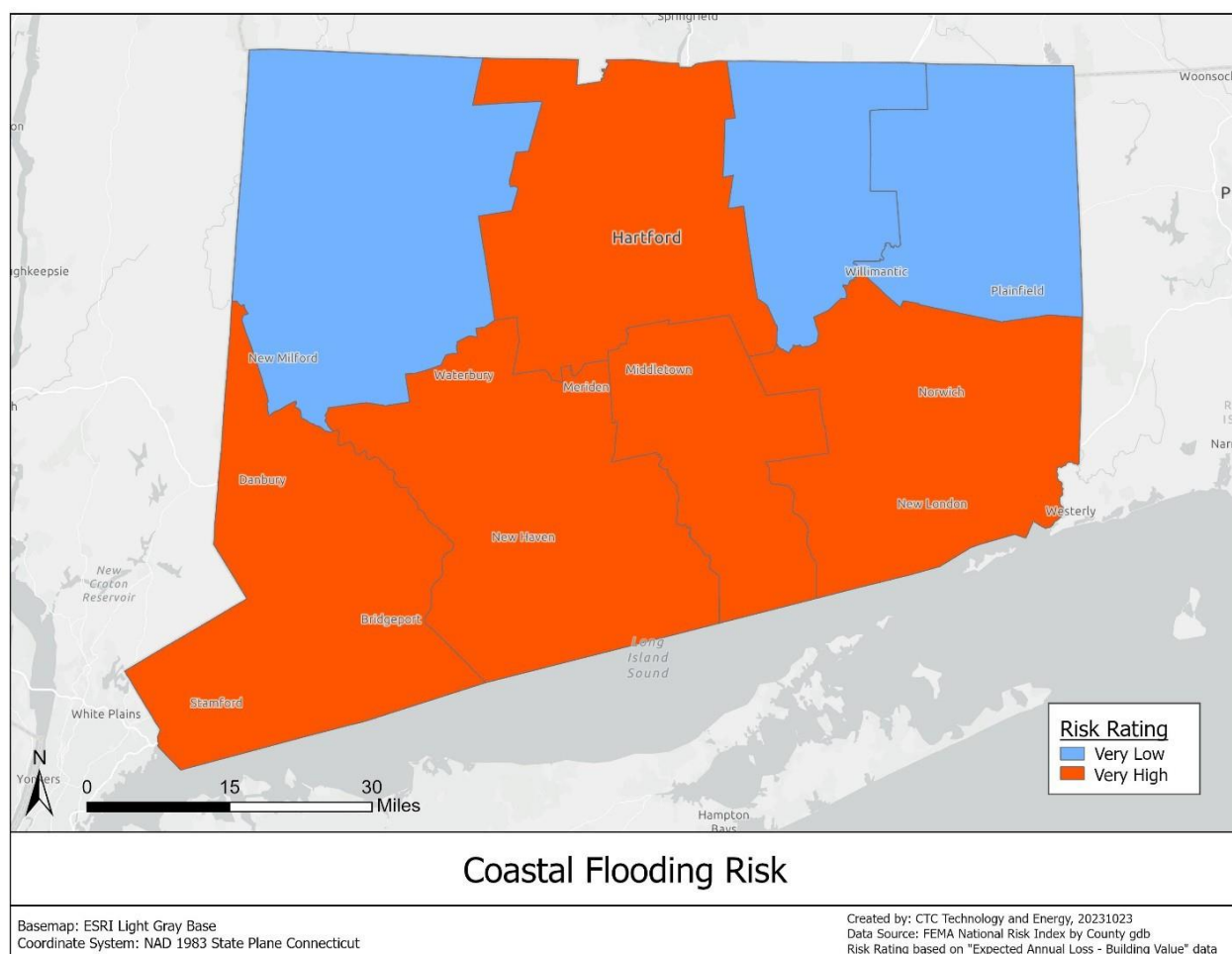
Figure 3: Coastal Flooding Risk in Connecticut
