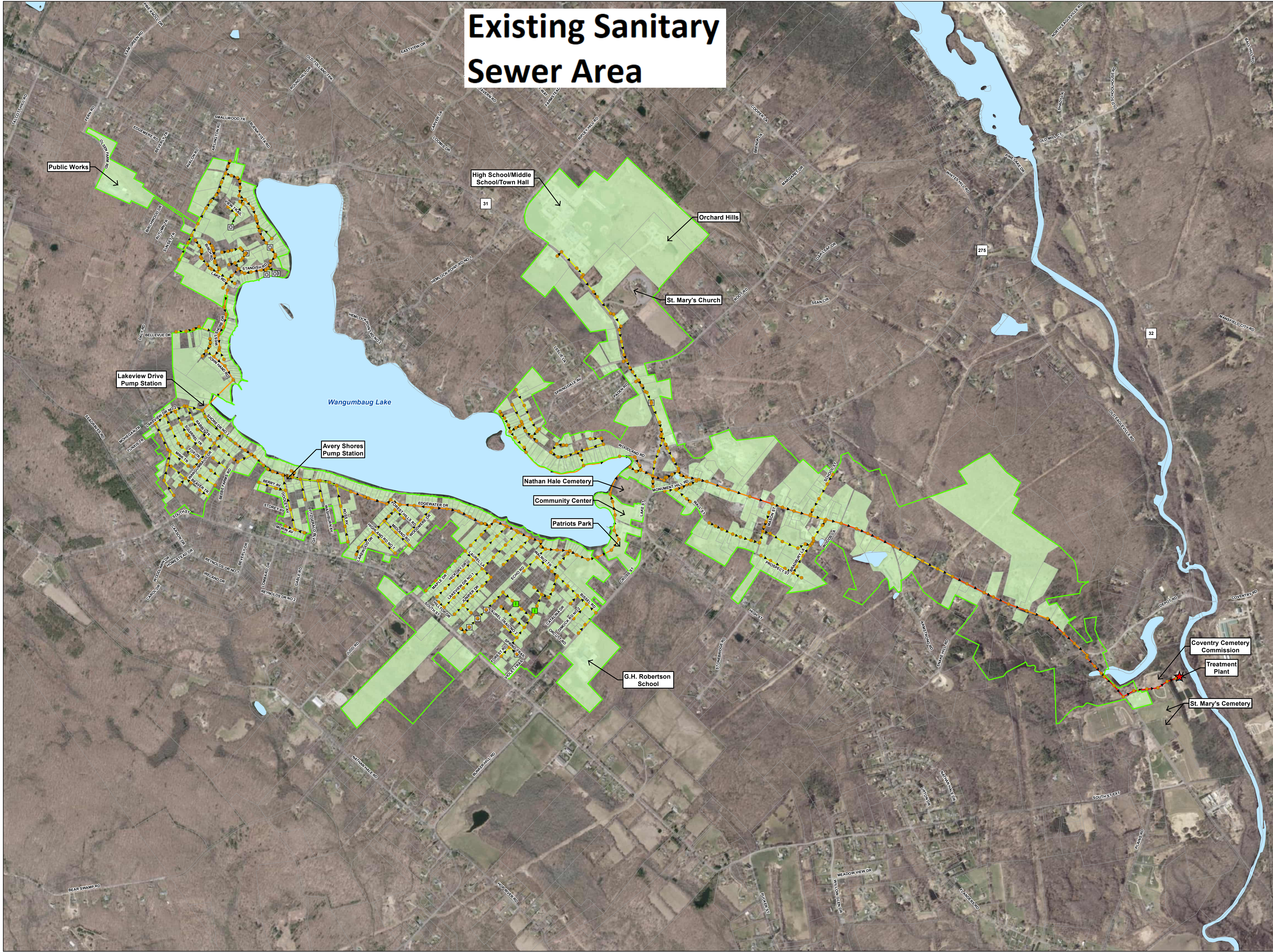
FIGURE 1 Existing Sanitary Sewer Service Area December 2023
