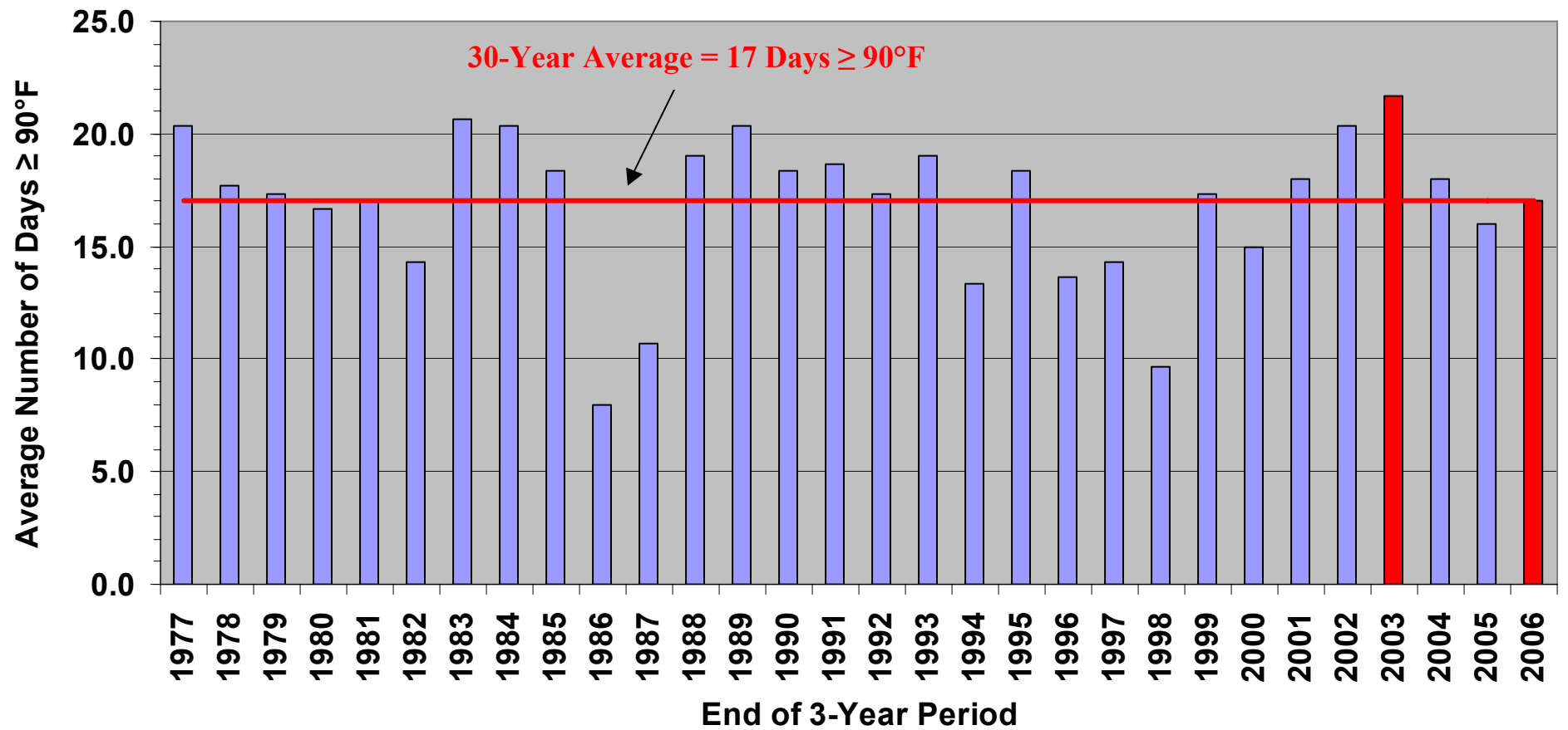
Figure 2-3 Number of Days with Maximum Temperature \geq 90^{\circ}\text{F} (3-Year Running Average at BDL)
