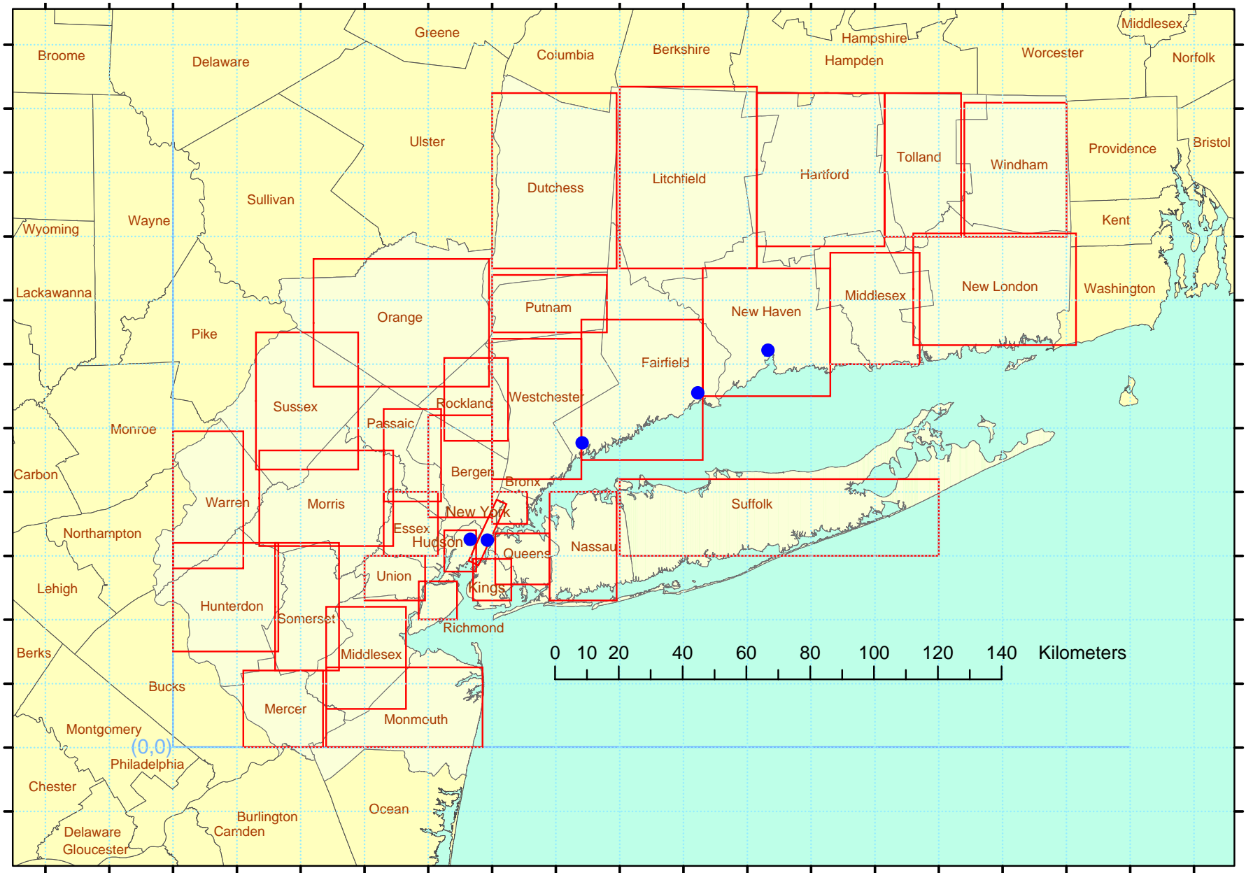
Figure 2-6: County-Based Area Sources Included in ISC Primary PM 2.5 Modeling
