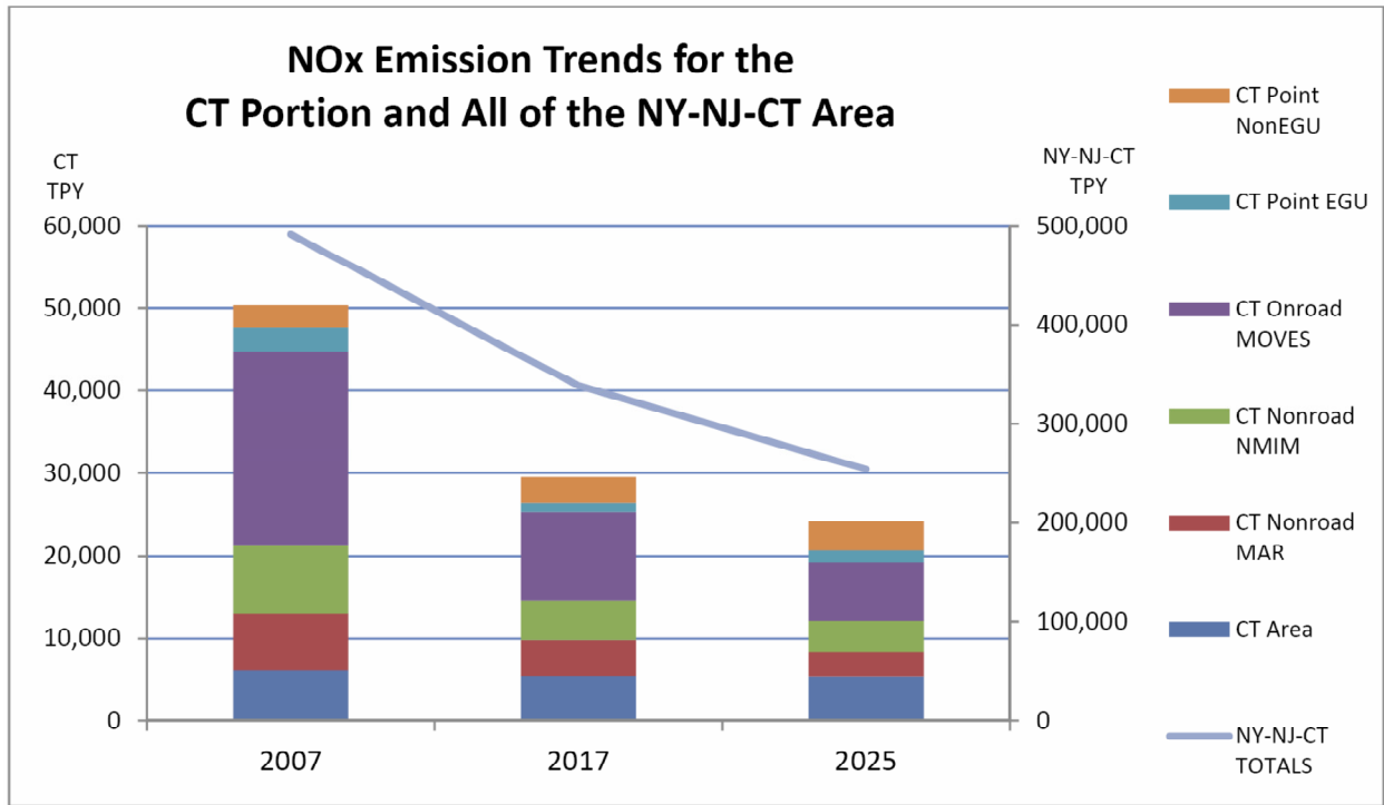
Figure 5. NOx Emission Projections 2007-2025
