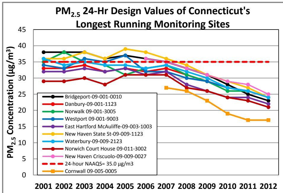
Figure 3. 24-hour PM_{2.5} Design Value Trends for Connecticut (2001-2012)
