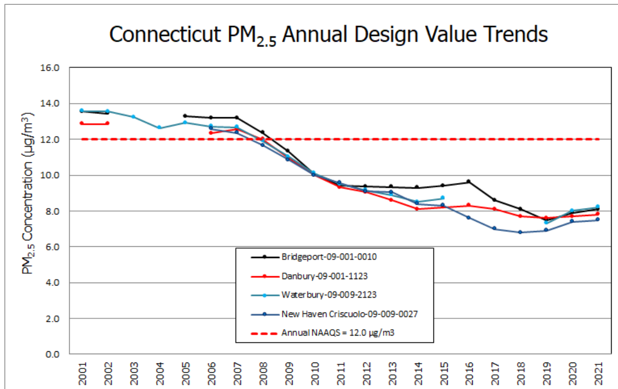
Figure 2-2. Annual Design Value Trends for Connecticut Monitors in the NY-NJ-CT Maintenance Area.
