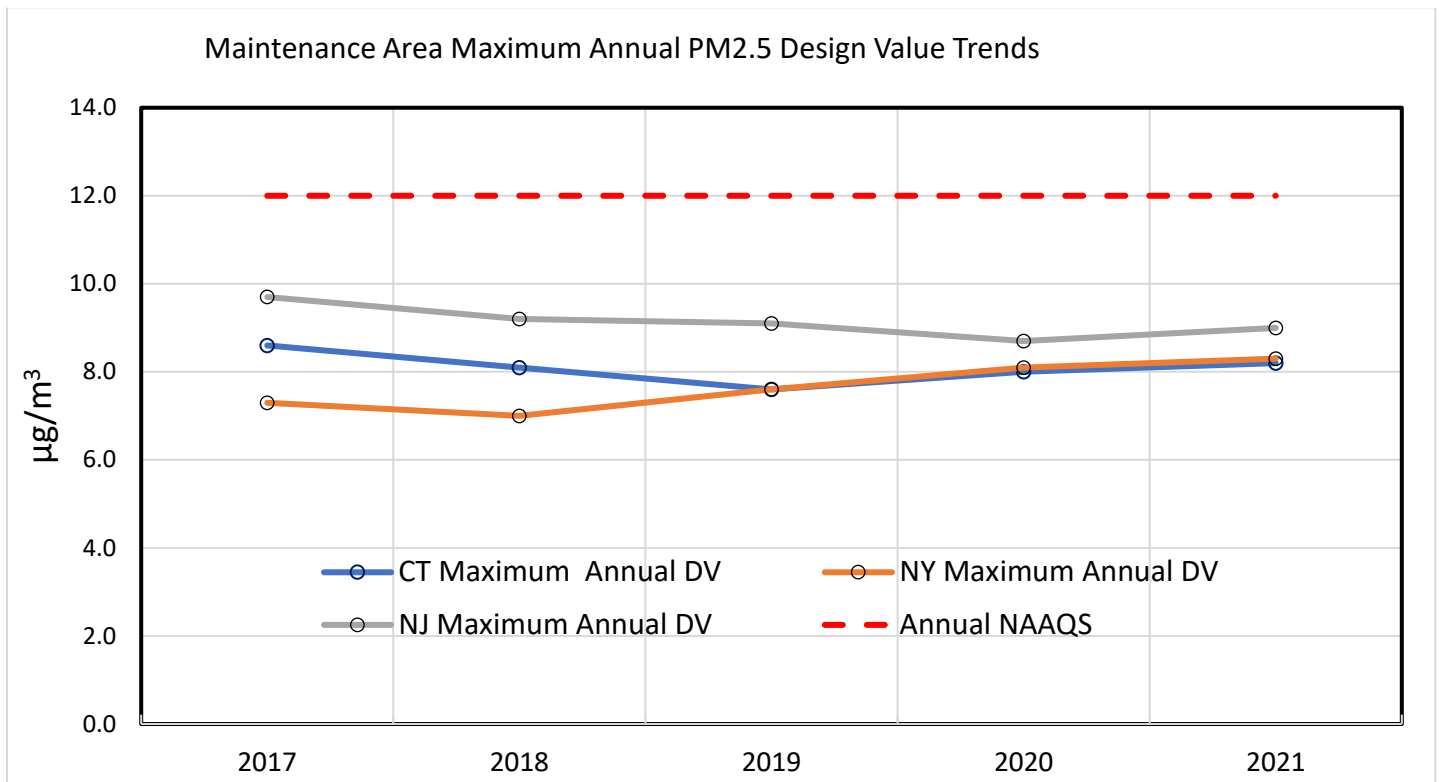
Figure 2-4. Maximum Annual Design Value for each State within the Maintenance Area (2017- 2021).
