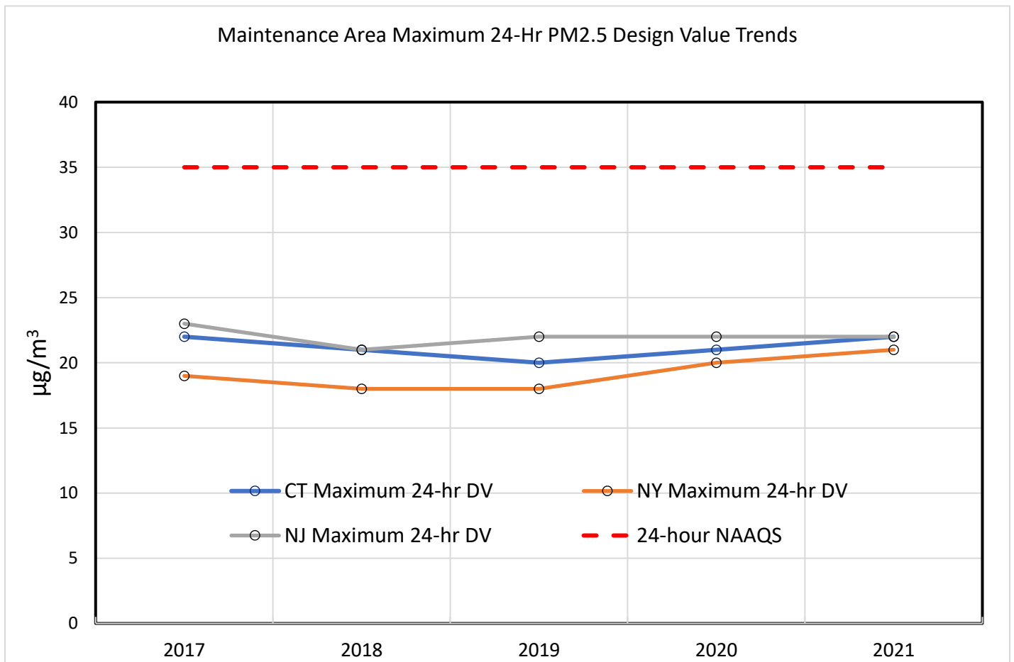
Figure 2-3. Maximum 24-Hour Design Value for each State within the Maintenance Area (2017-2021).
