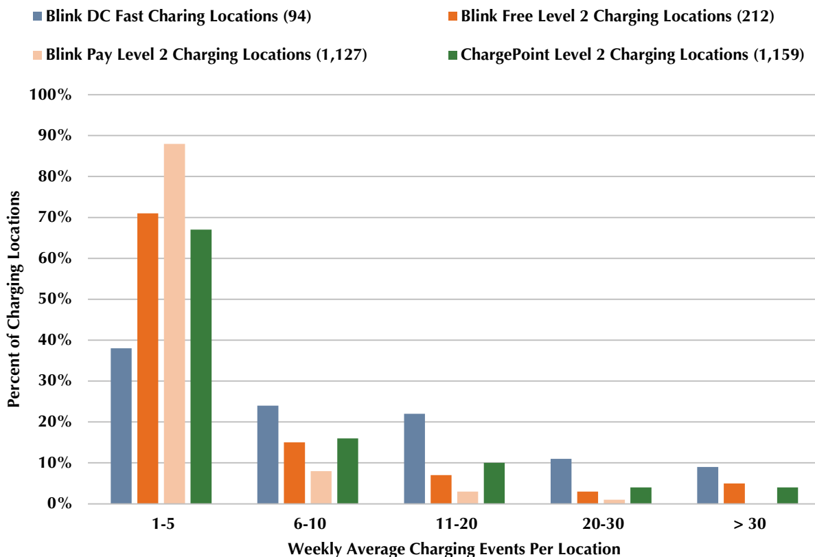
FIGURE 12: Charging Use for the EV Project
