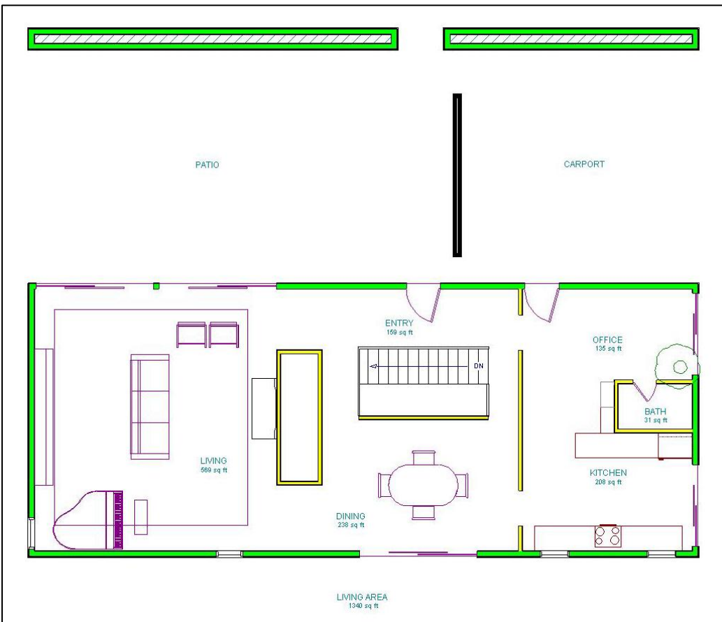
Figure 11. Plans of the Becker House provided by the current owner.
