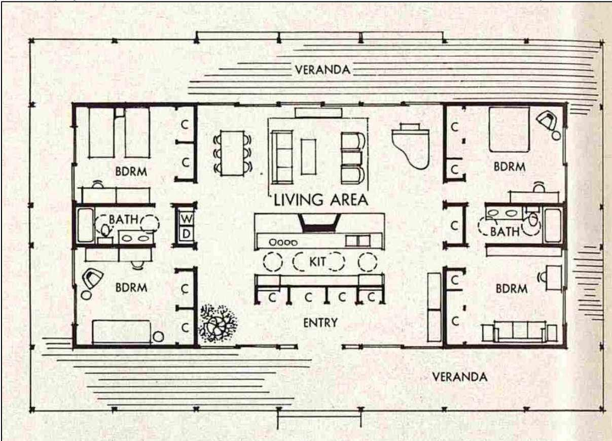
Figure 18. The plan of JBL II as originally constructed (Better Homes & Gardens, October 1958).
