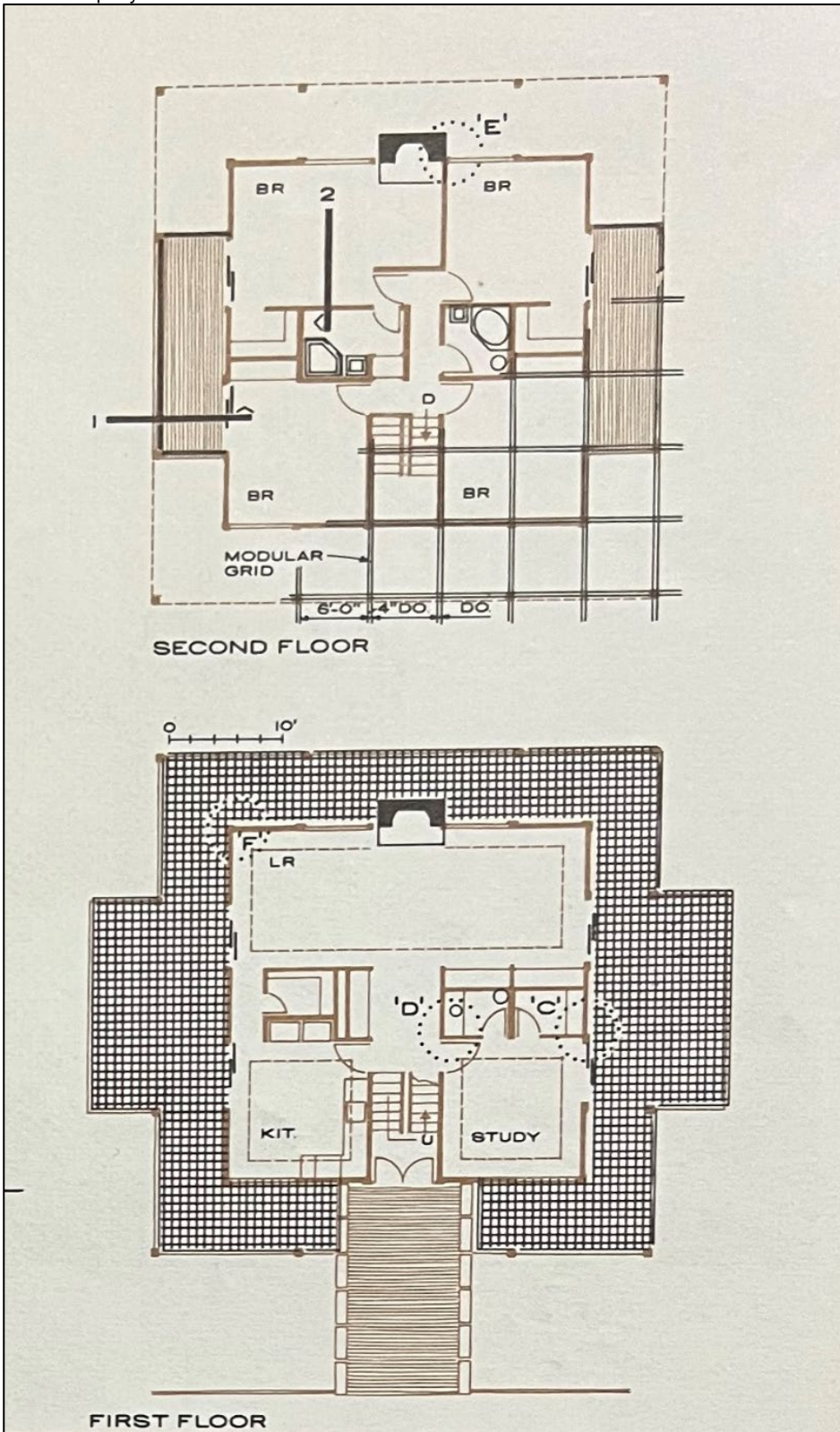
Figure 7. Plan of the System House as published in Progressive Architecture .
