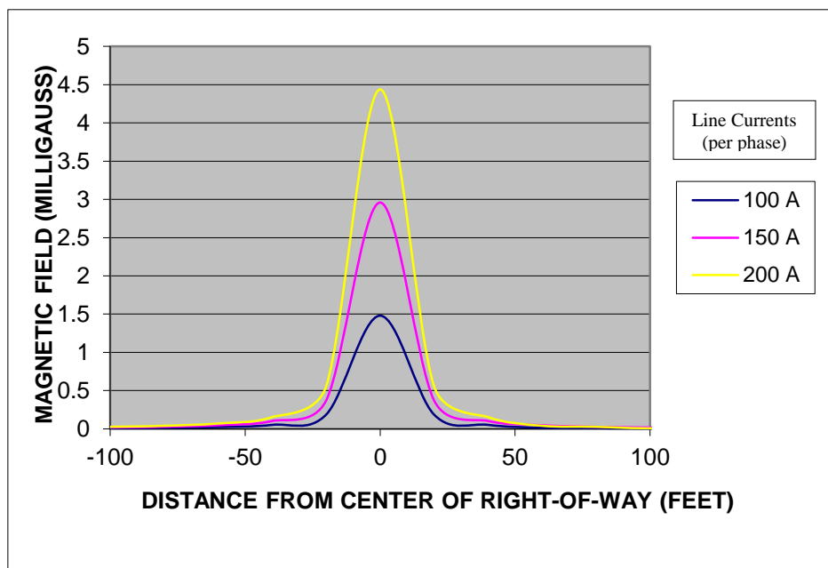
Figure E-3: Magnetic Field Profiles for Typical 345 kV HPFF Line*
