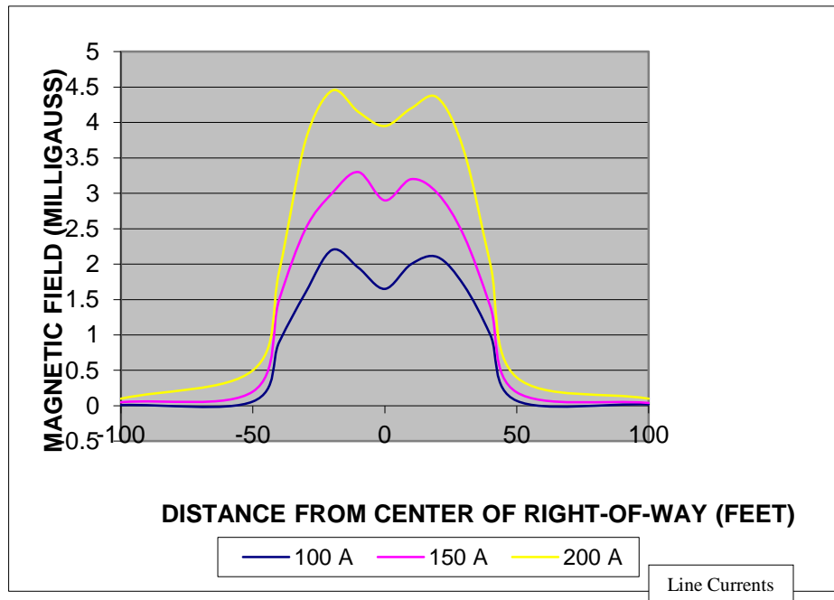
Figure 7-2: Average of Magnetic Field Measurements for 345 kV HPFF Line*
