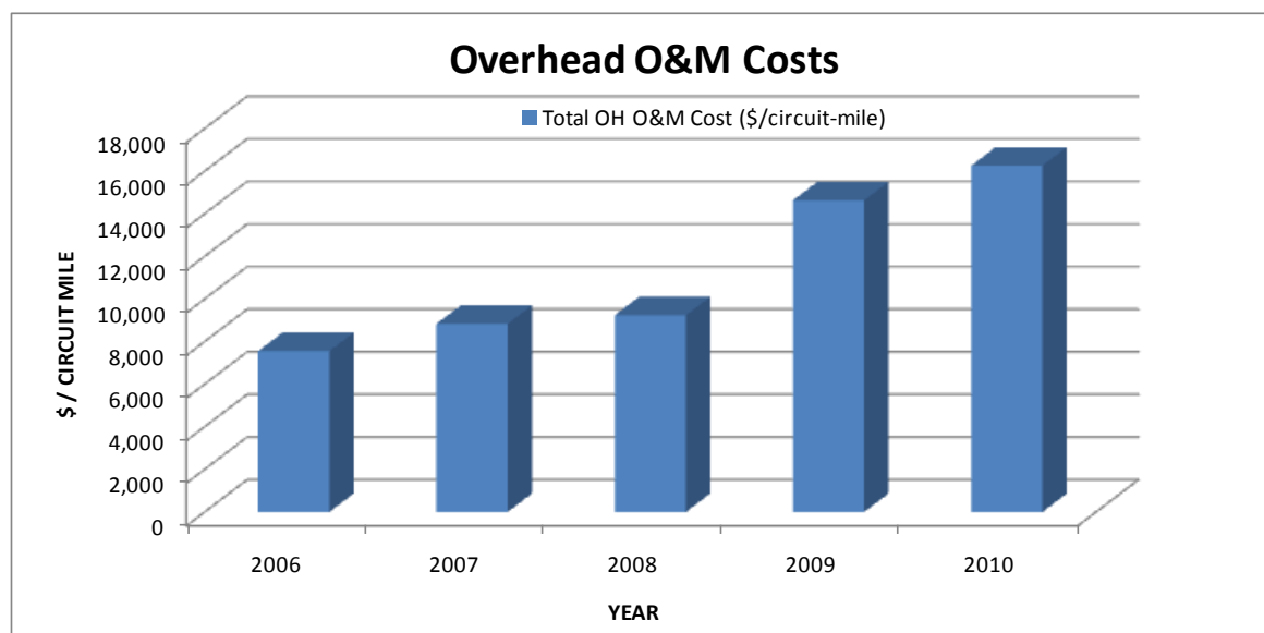
Figure 6-1: Total Overhead Transmission Line O&M Costs, 2006-2010
