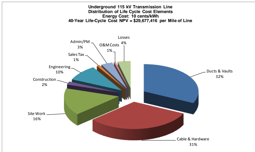
Figure 1-3: Life-Cycle Costs for a Typical 115 kV Underground Line
