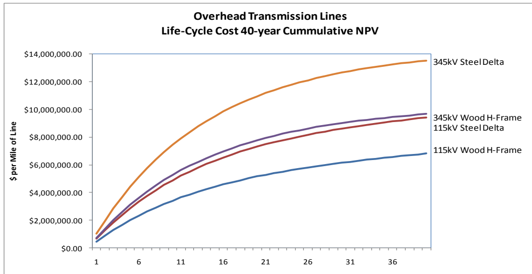
Figure 9-1: Overhead Transmission Line Life-Cycle Costs
