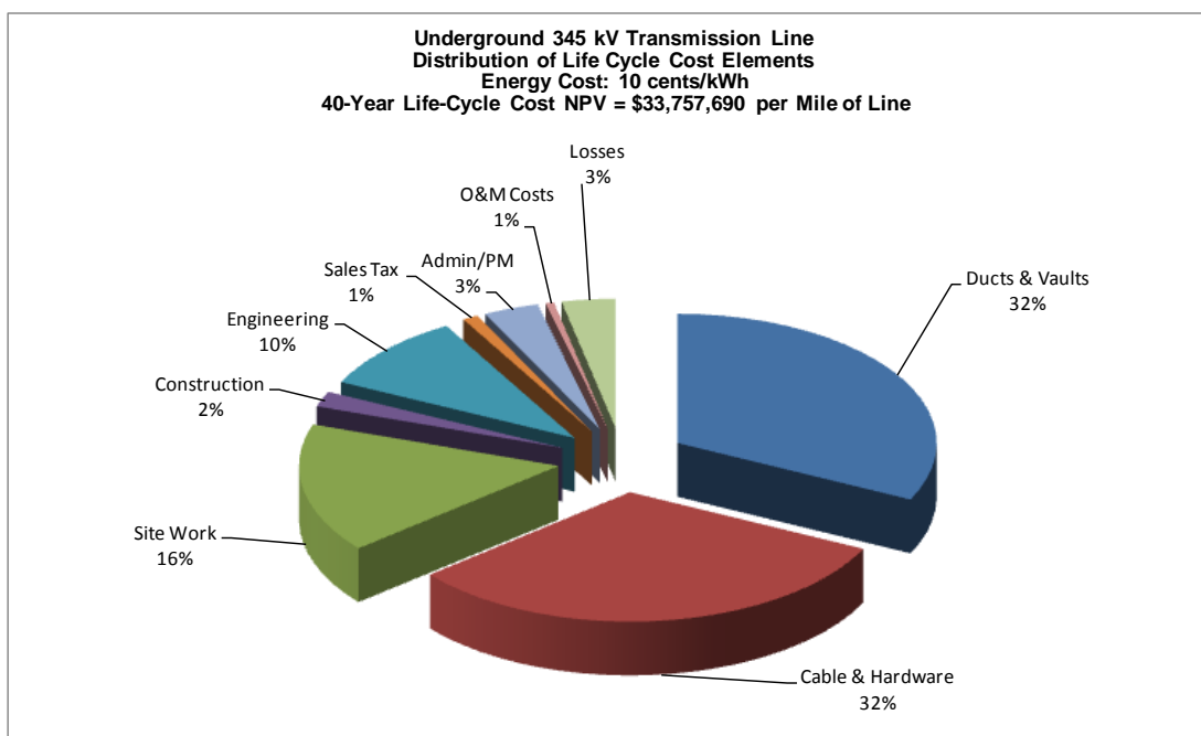
Figure 1-4: Life-Cycle Costs for a Typical 345 kV Underground Line
