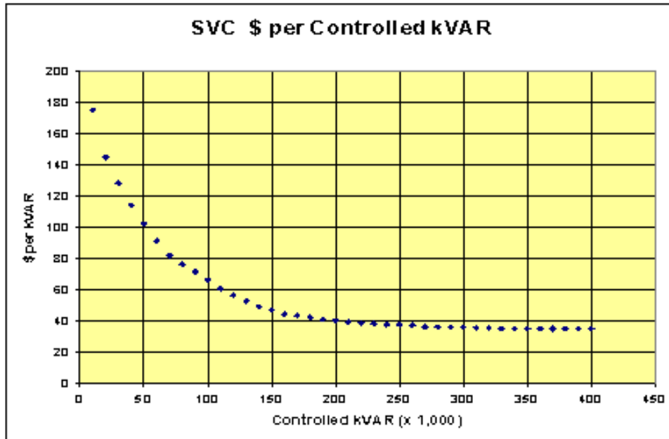
Figure 4-1: SVC System Cost vs. Size (Controlled kVAR)
