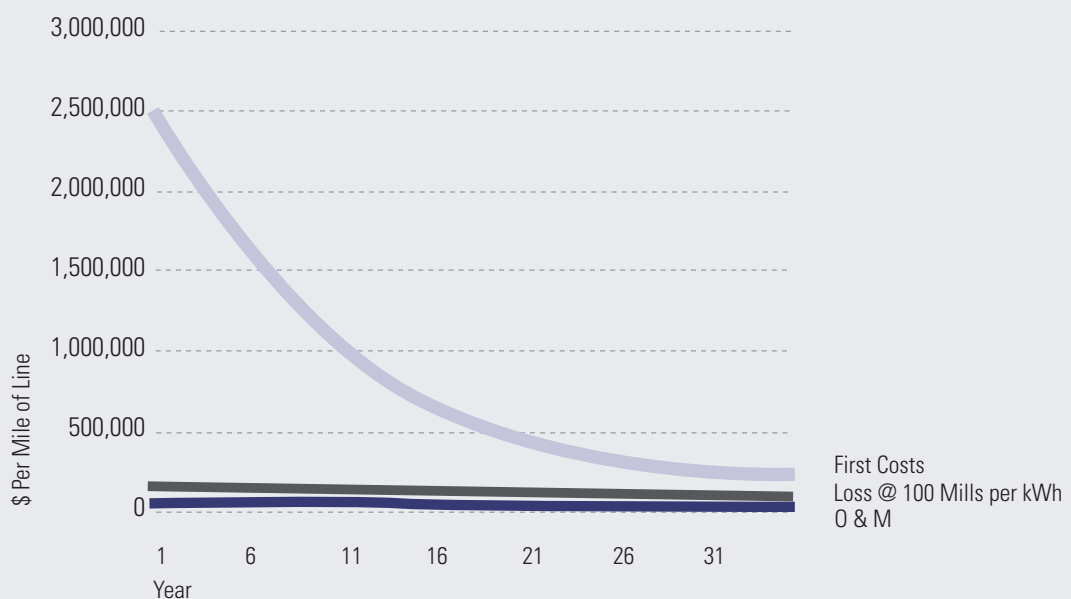
Figure 10.6. 345 kV Underground Transmission Line Component Costs
