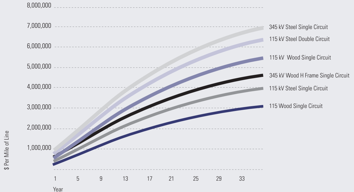
Figure 10.1. Overhead Transmission Line Life Cycle Costs
