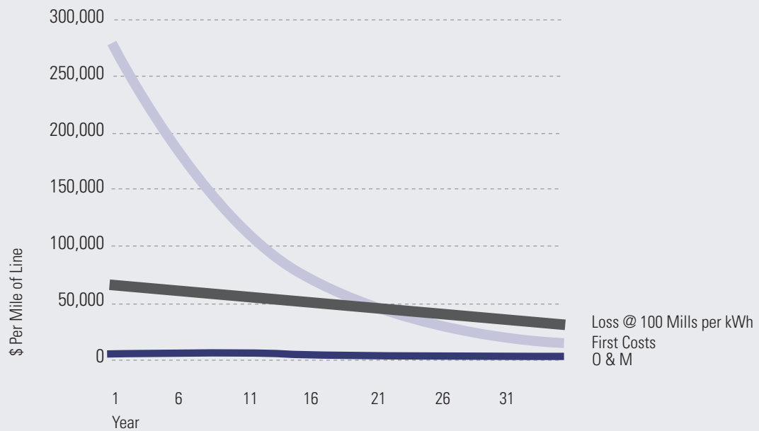
Figure 10.5. 345 kV Overhead Transmission Line Cost Components
