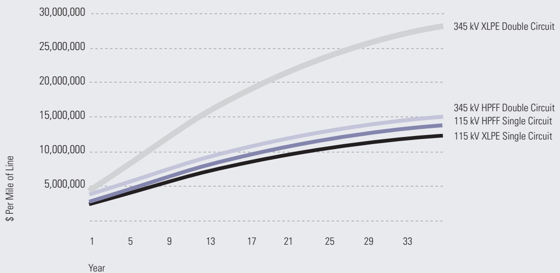
Figure 10.2. Underground Transmission Line Life Cycle Costs
