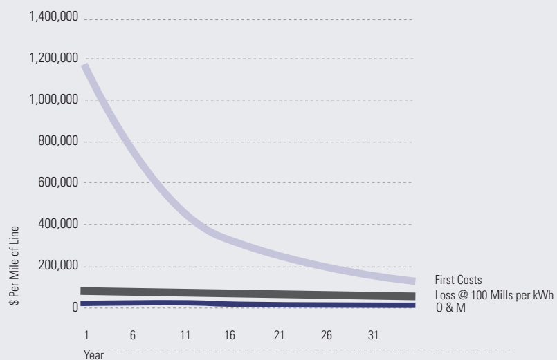
Figure 10.4. 115 kV Underground Transmission Line Component Costs
