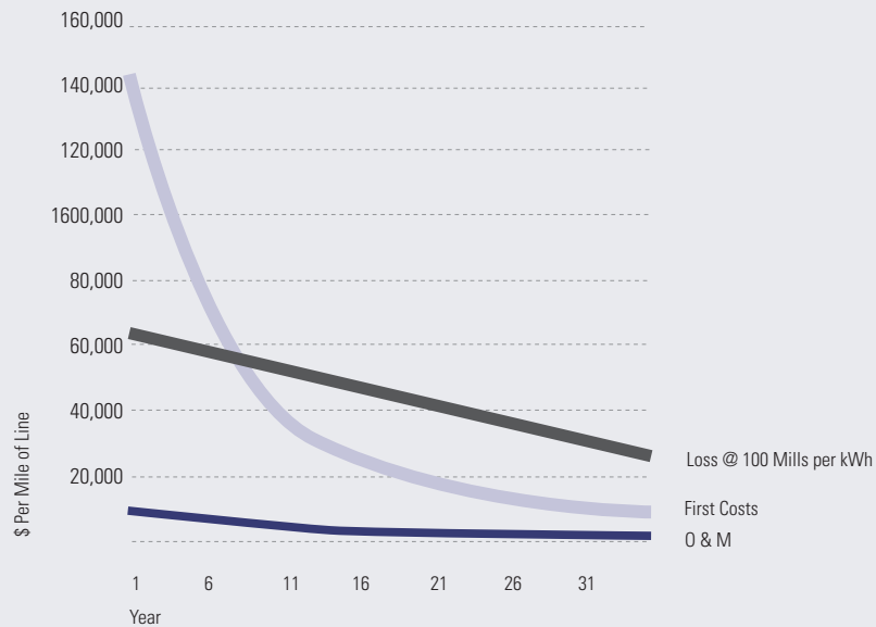
Figure 10.3. 115 kV Overhead Transmission Line Component Costs
