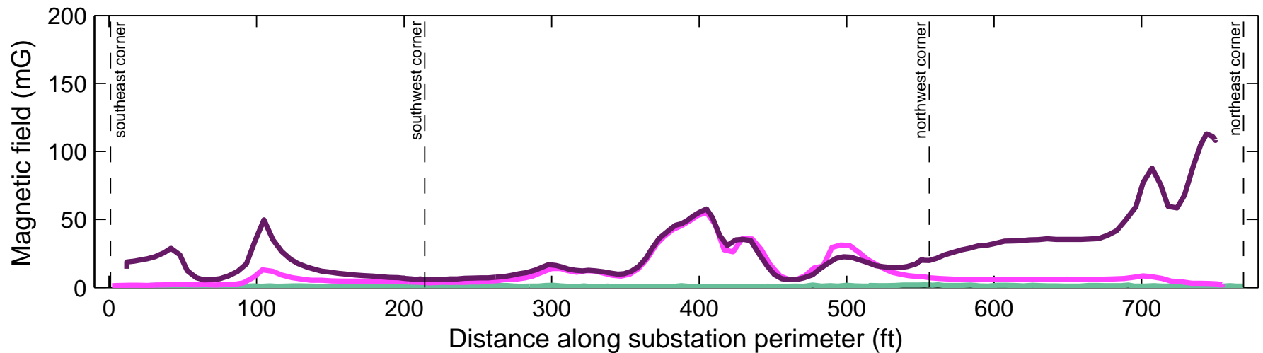
EMF measurements along the perimeter of the Singer Substation
