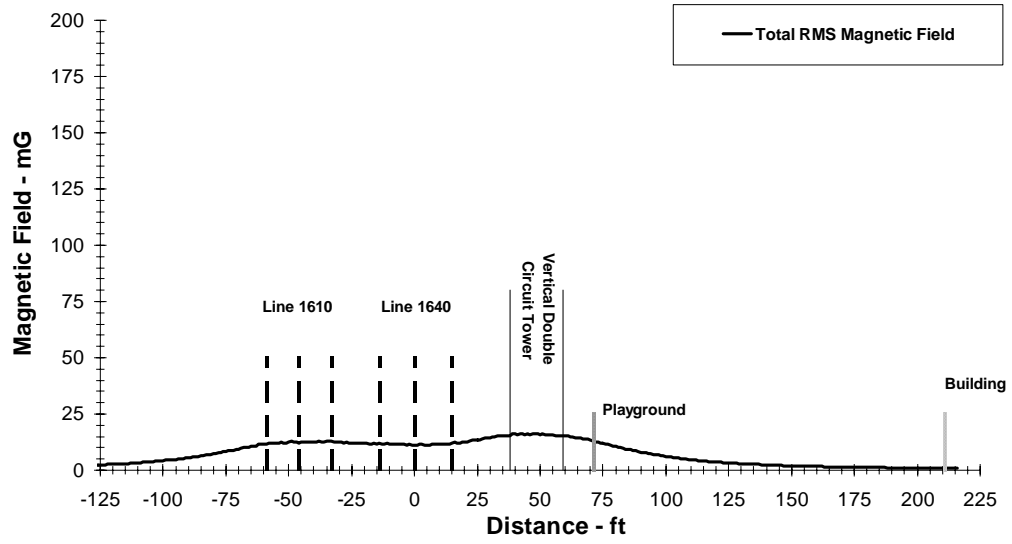
Figure 3. Magnetic field profile from south to north for the transmission lines adjacent to the High Plains Community Center in Orange
