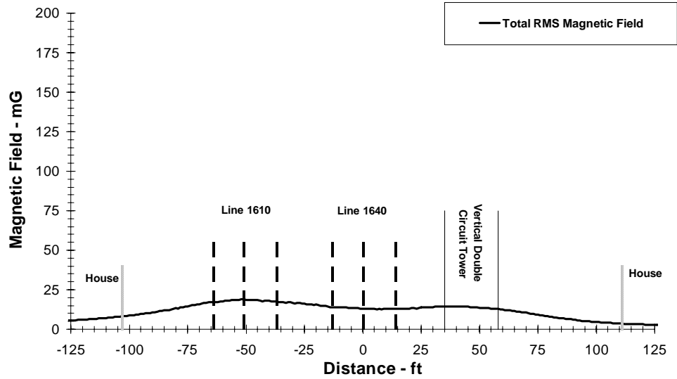
Figure 1. Magnetic field profile from south to north for the transmission lines passing over Route 114 (Center Road) in Woodbridge
