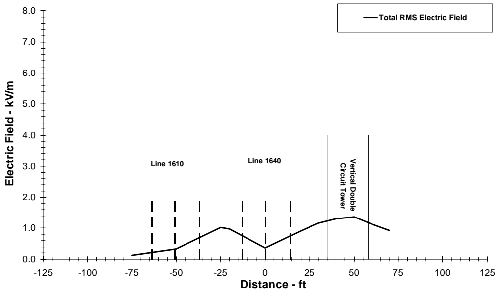
Figure 2. Electric field profile from south to north for the transmission lines passing over Route 114 (Center Road) in Woodbridge
