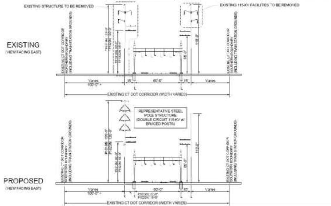
Figure 12 –Allings Crossing Substation to Elmwest Substation Structure Nos. P1019N to P1020N – Cross Section
