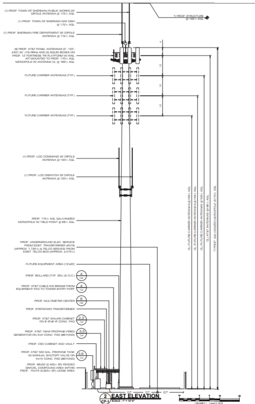
Figure 6: Compound/tower profile
