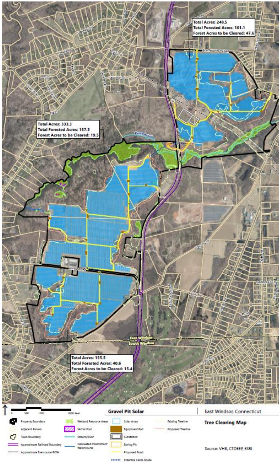
Figure 7 – Site Clearing
