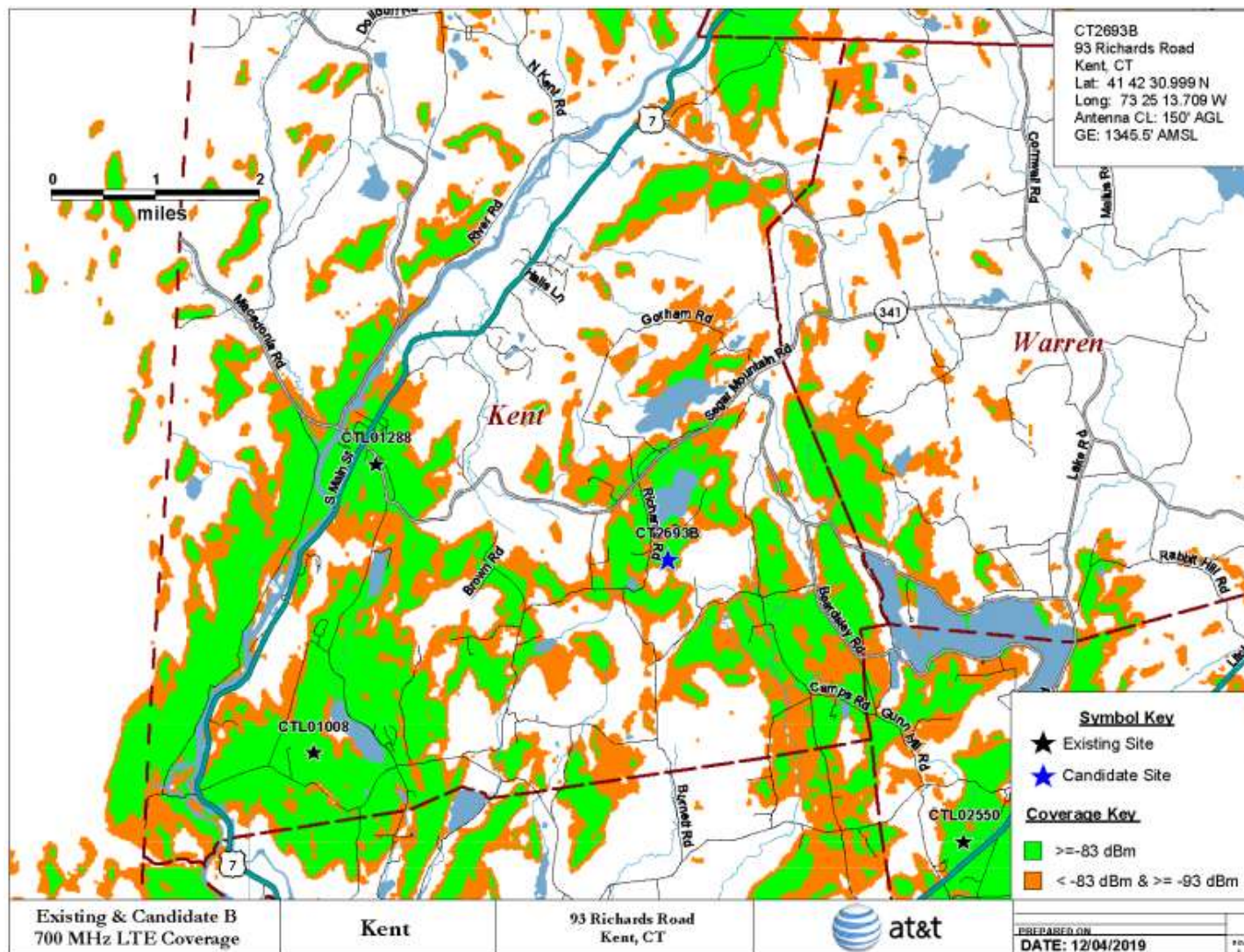
Figure 5 – Site B Existing and Proposed 700 MHz Service (Antennas at 150 feet)
