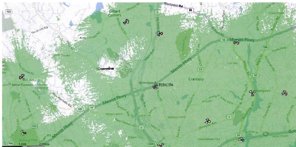
Figure 16 – Existing and Proposed Sprint 1900 MHz Coverage
