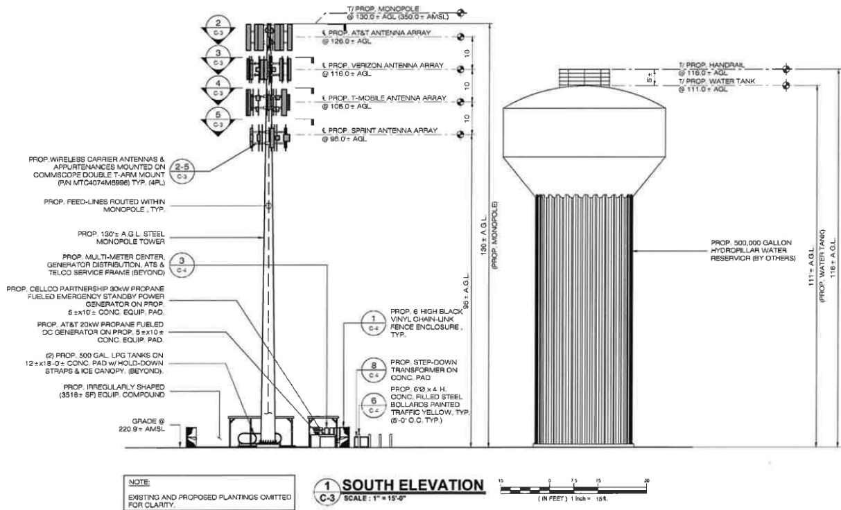
Figure 4 – Tower Profile Drawing
