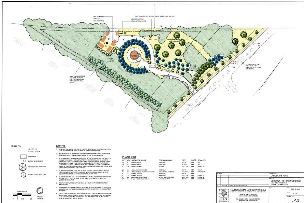
Figure 3 – Landscaping Plan
