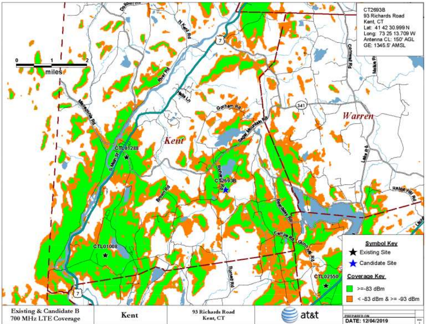
Figure 5 – Site B Existing and Proposed 700 MHz Service (150 feet)
