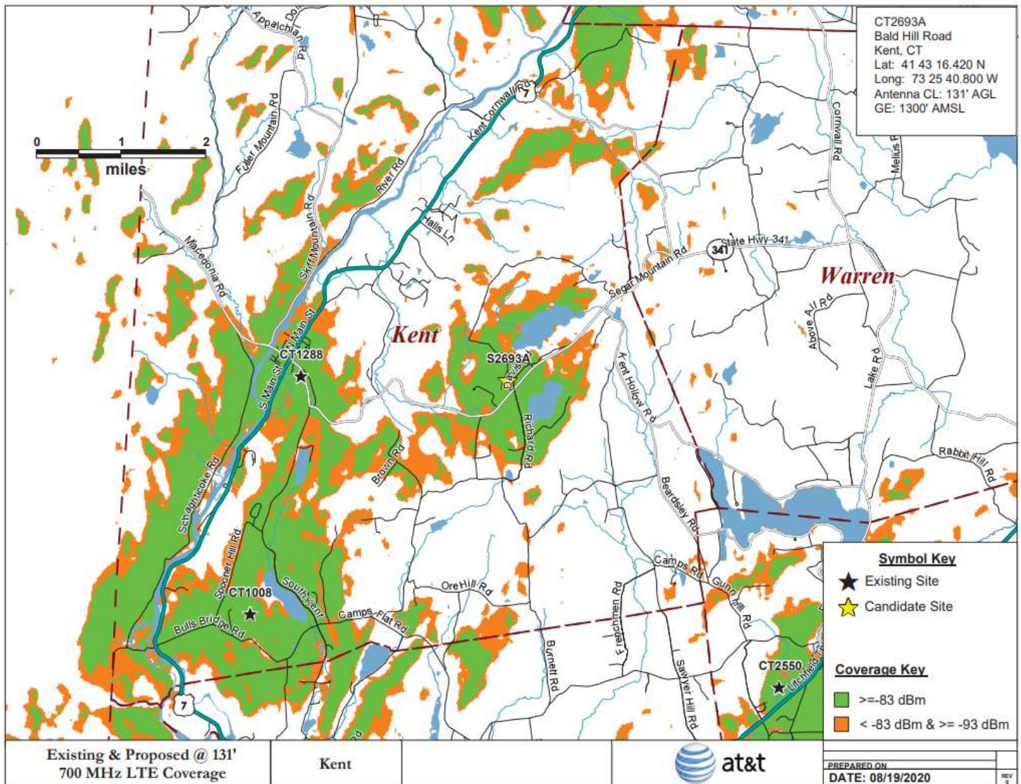
Figure 6 – Site A Existing Proposed 700 MHz Service (131 feet)
