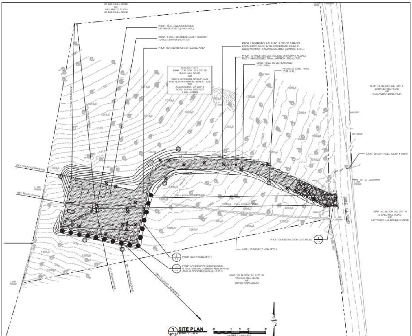
Figure 11 – Site A – Site Plan
