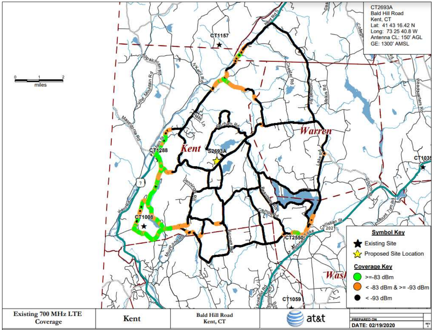
Figure 3 – Drive Test Data Showing Existing 700 MHz Service
