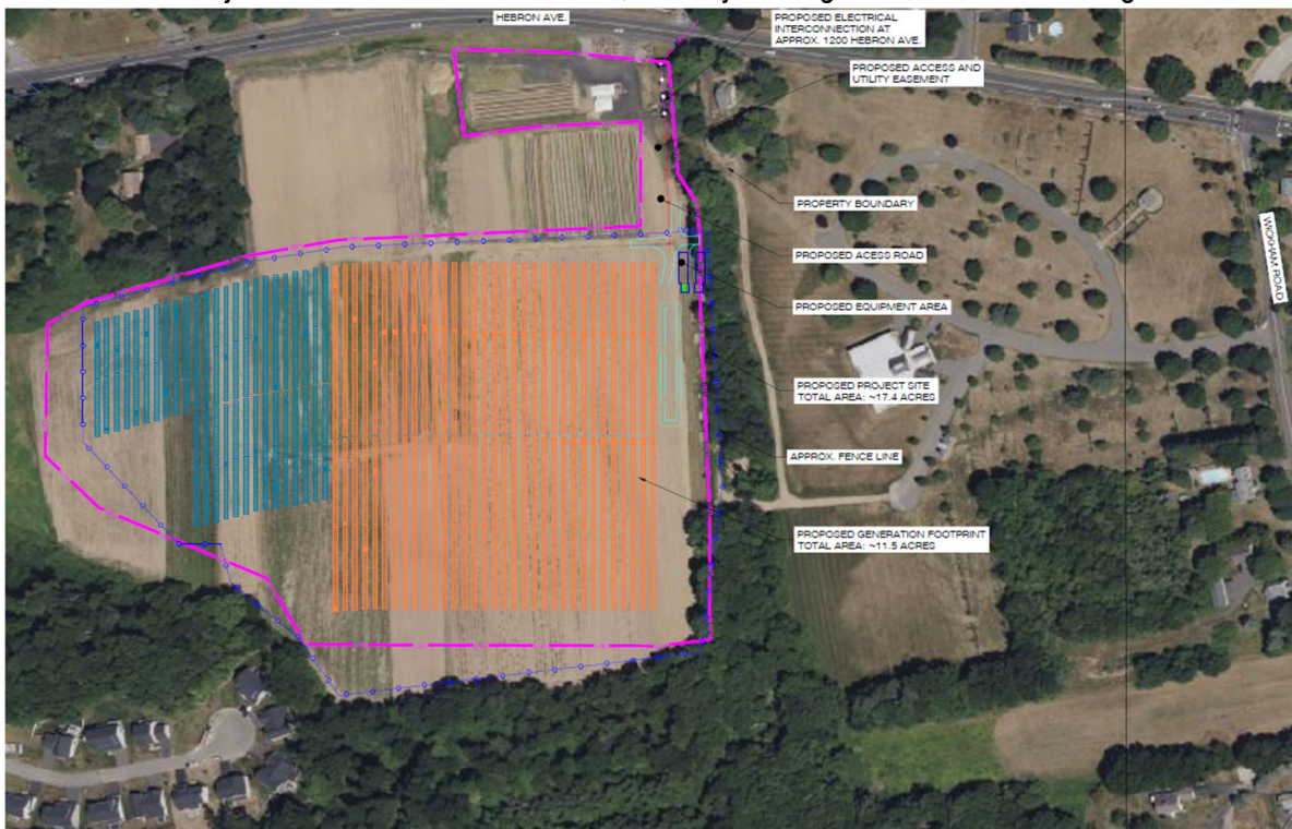
GLASTONBURY SOLAR ONE - SITE PLAN SCALE: 1" = 80'
