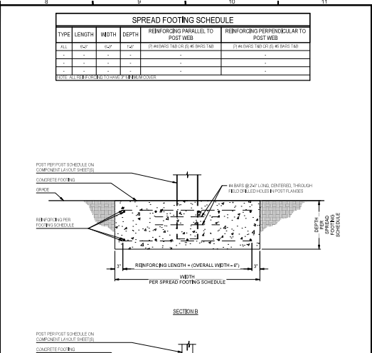
A8 ALTERNATE FOUNDATION SPREAD FOOTING DETAIL
