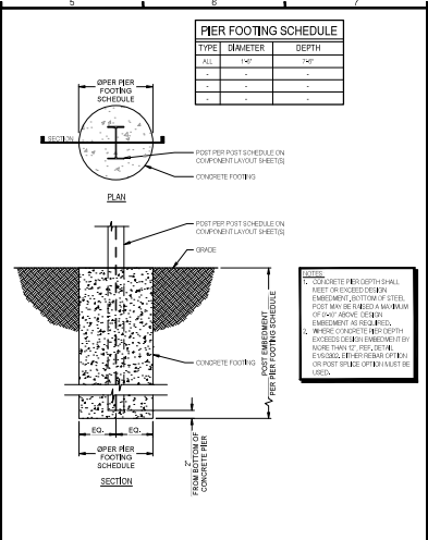
E2 ALTERNATE FOUNDATION PIER FOOTING DETAIL
