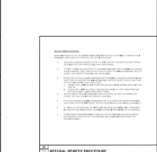
A2 REFUSAL REMEDY PROCEDURE
