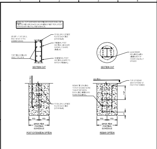
E1 ADDITIONAL PIER FOOTING DETAIL WHEN EMBED EXCEED DESIGN
