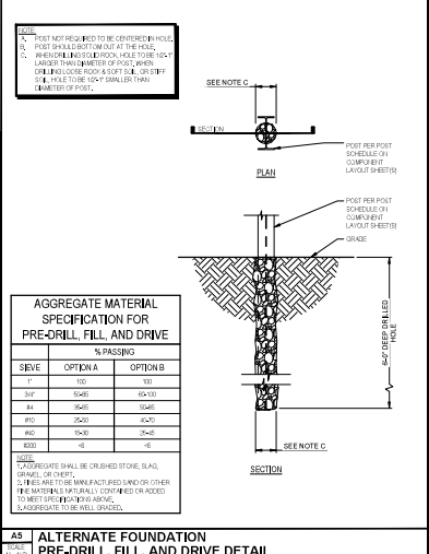
A5 ALTERNATE FOUNDATION PRE-DRILL, FILL, AND DRIVE DETAIL
