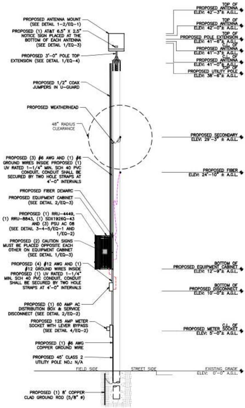
① POLE ELEVATION SCALE: 3/16" = 1'-0"
