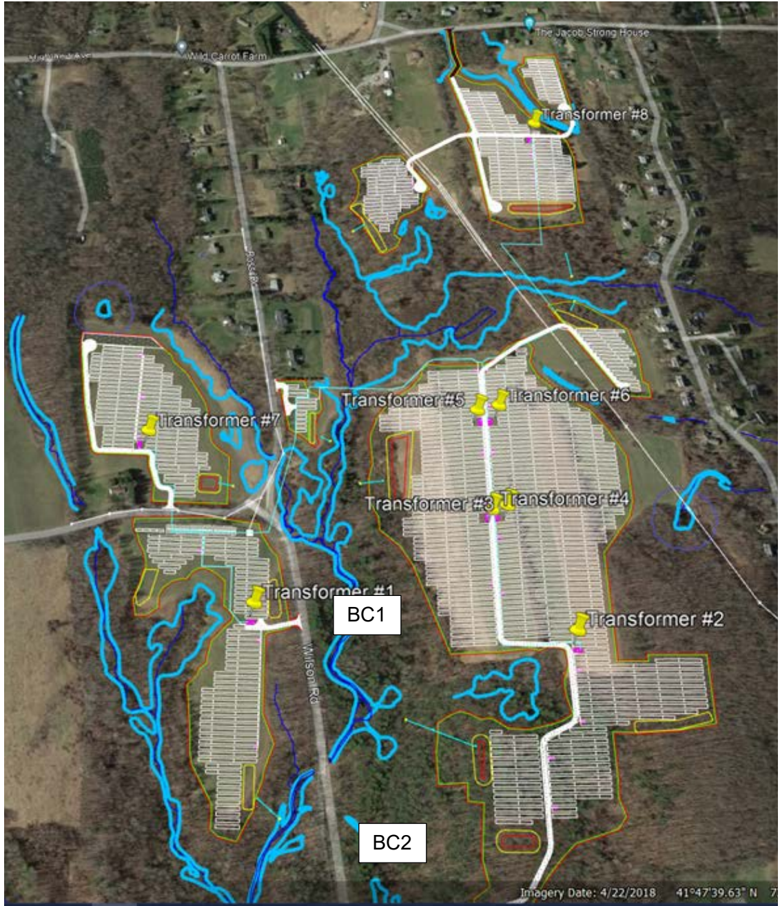
Figure C-2: Site plan
