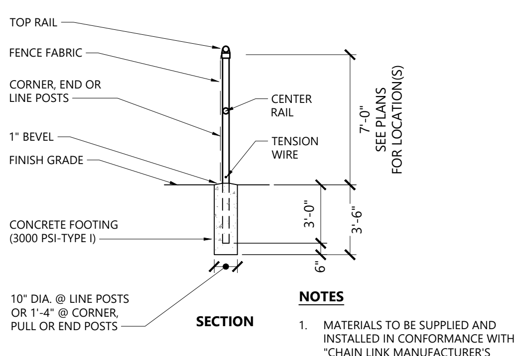
7' Chain Link Fence with Privacy Slats 1/16 N.T.S. Source: VHB LD_480
