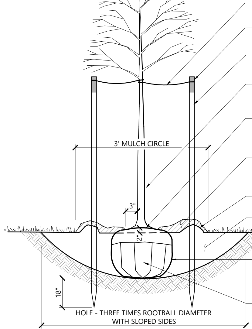
Tree Planting (For Trees Under 4" Caliper) 9/18 N.T.S. Source: VHB LD_602
