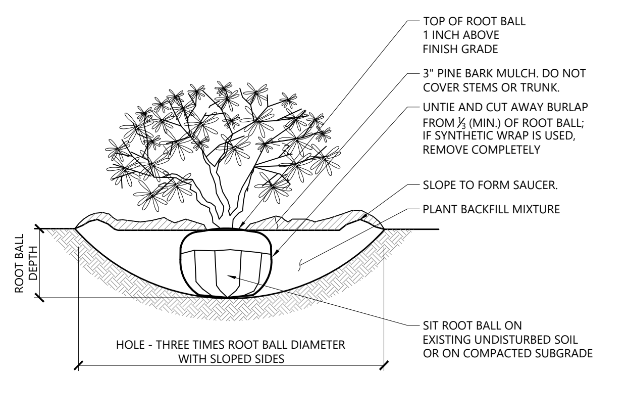
Evergreen Tree Planting 1/16 N.T.S. Source: VHB LD_604
