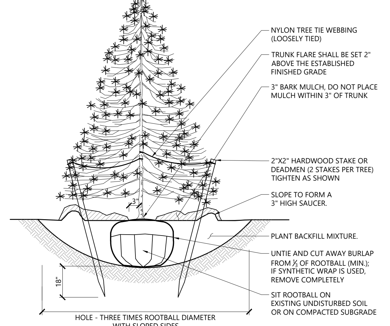
Evergreen Tree Planting 1/16 N.T.S. Source: VHB LD_604
