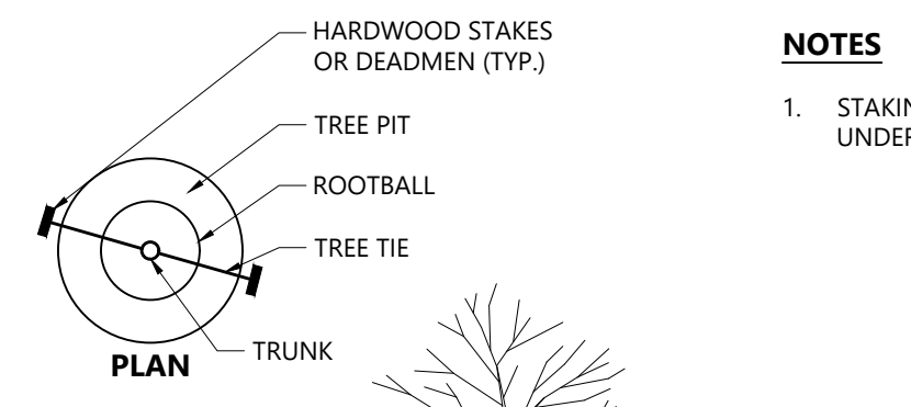
Evergreen Tree Planting 1/16 N.T.S. Source: VHB LD_604
