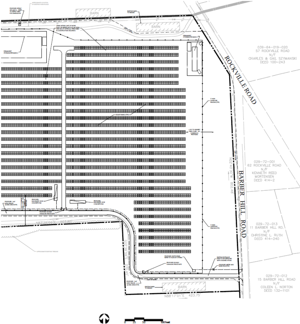
(GCE 3, Tab A – Revised Site Plans, Drawing No. C-3.2)
