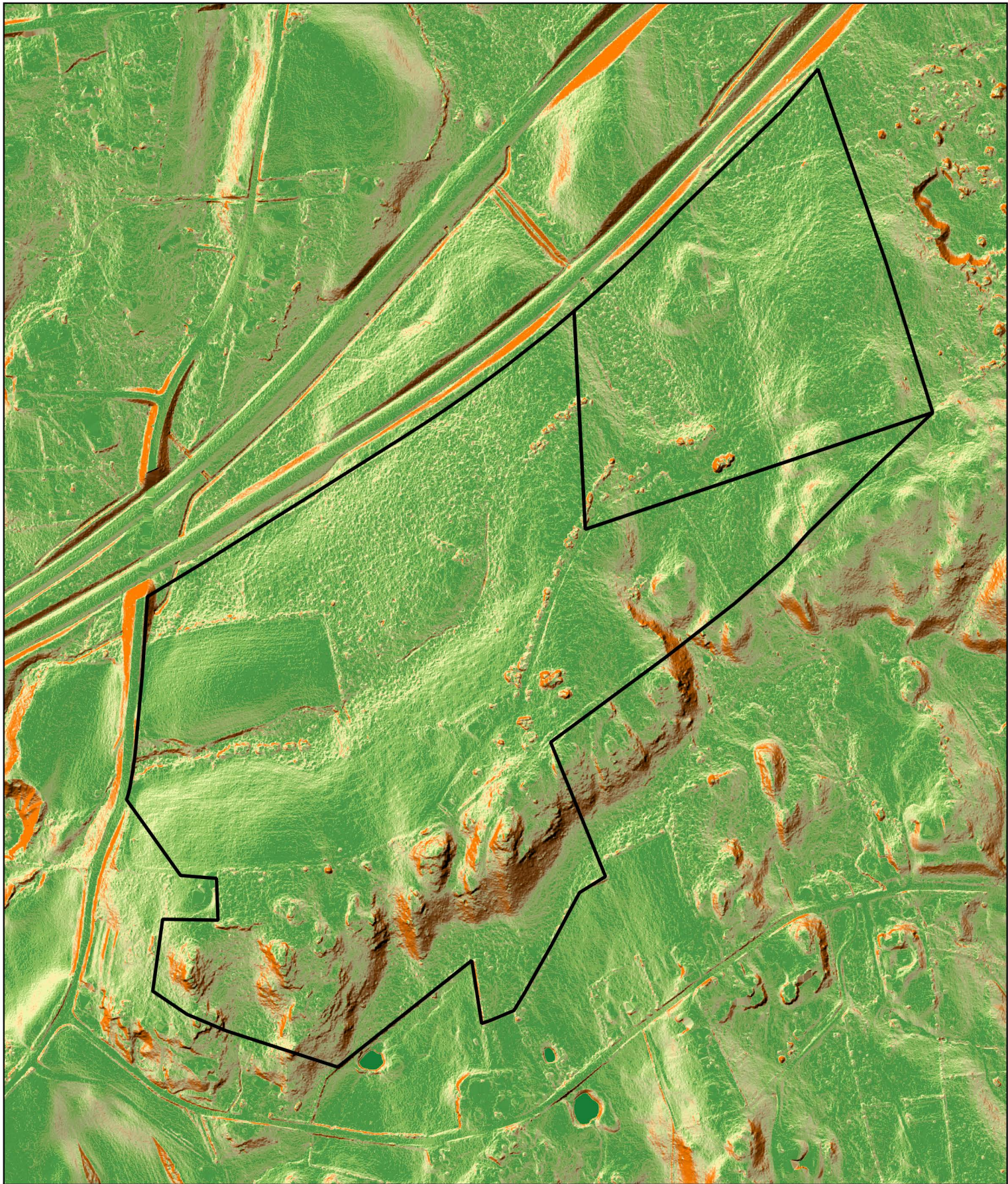
Figure 7 - SLOPE PERCENT RISE 227 BOOM BRIDGE RD, NORTH STONINGTON CT
