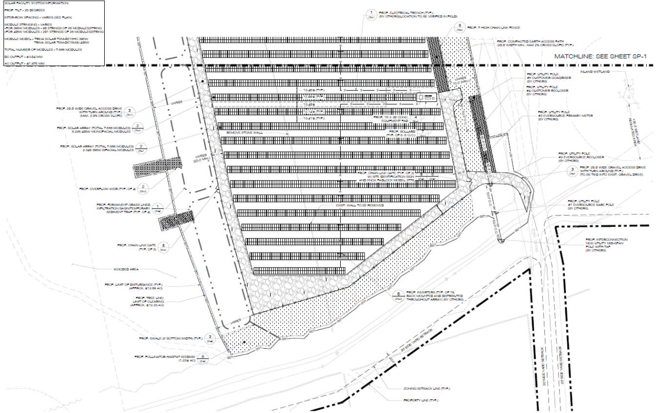
SITE & UTILITY PLAN SCALE: 1" = 60'-0" 10,000' 100,000'
