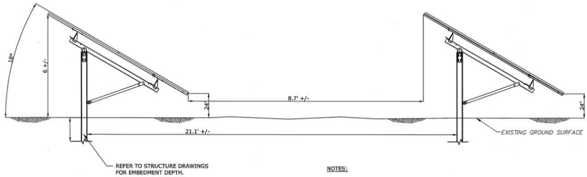
Figure 2 – Proposed Solar Rack Side Elevation View
