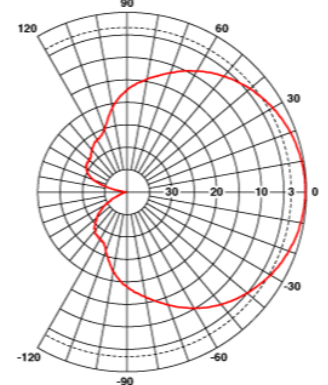
Horizontal Pattern
