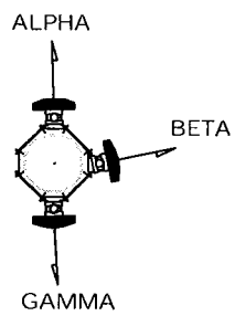
ANTENNA PLAN SCALE: 3/16" = 1'-0"
