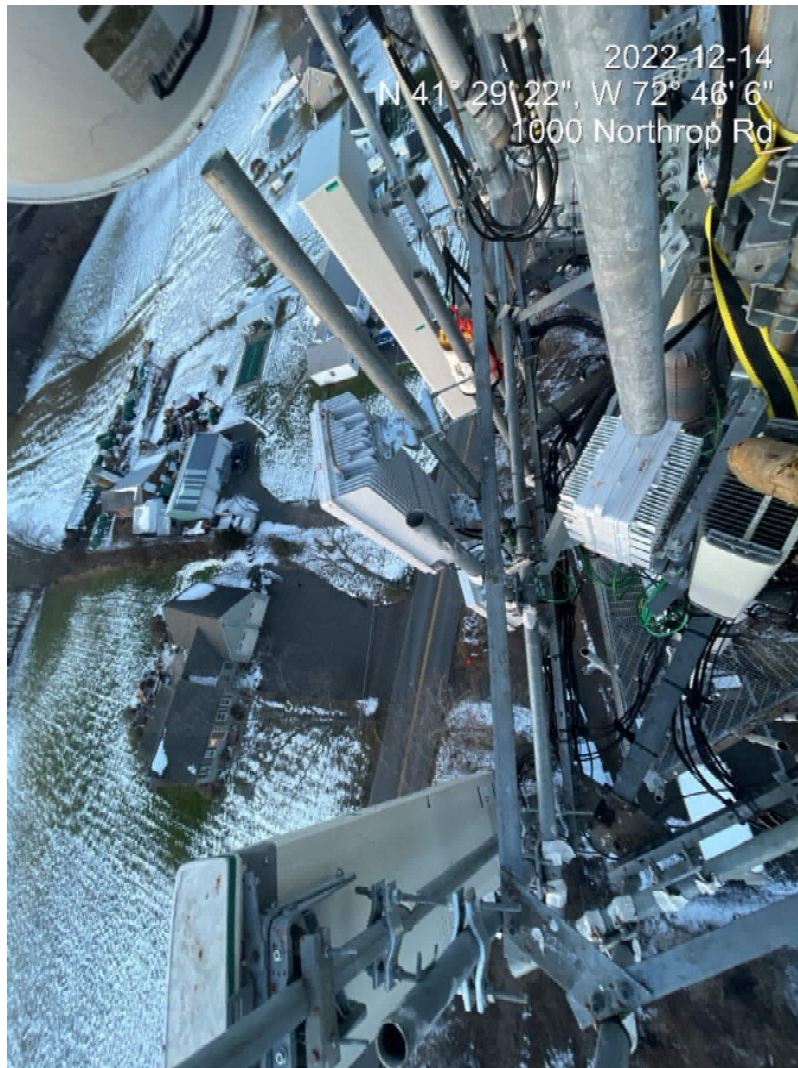
Photo - 3: Installation of antennas and remote radio heads, Gama Sector
