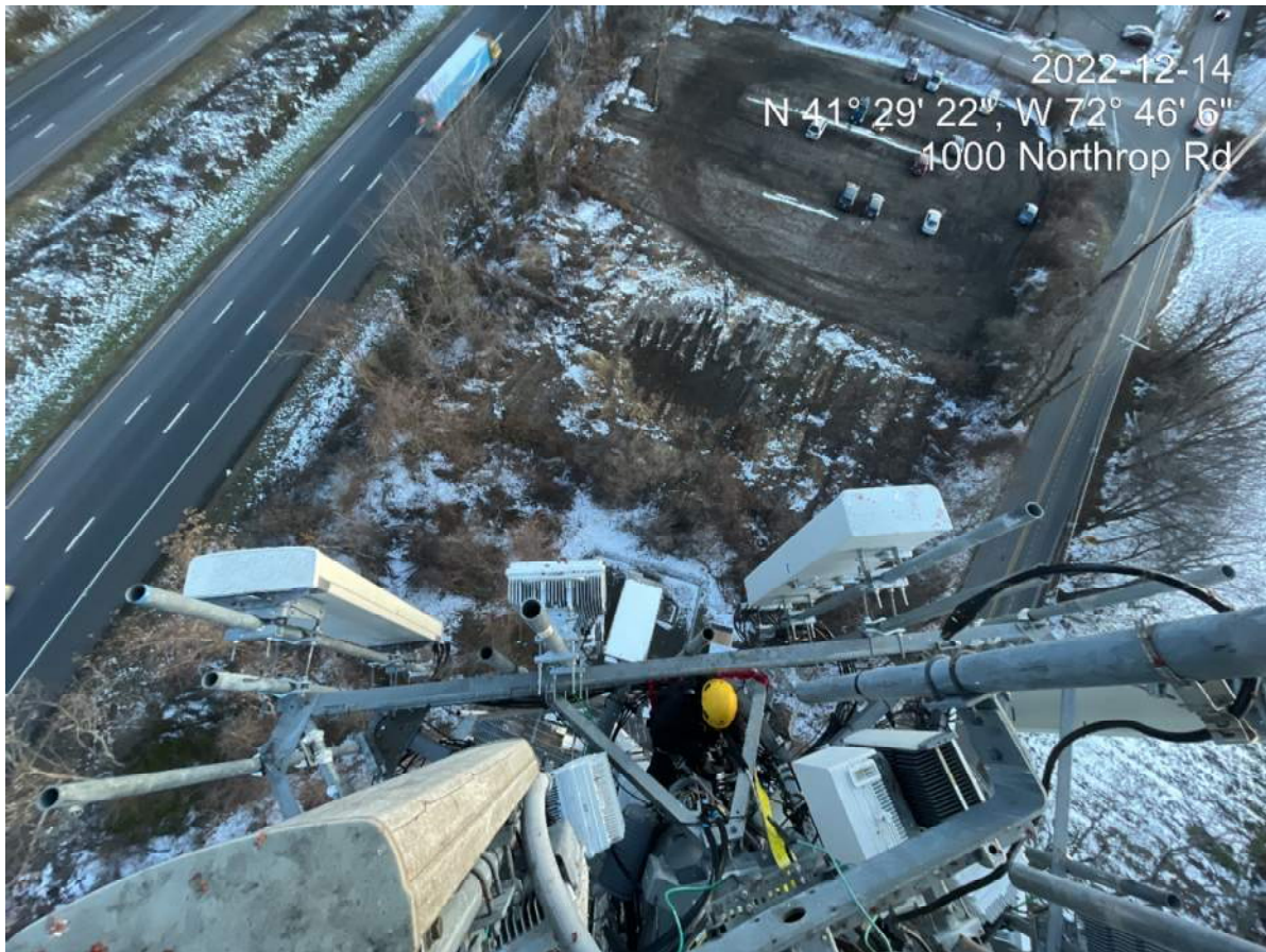
Photo - 2: Installation of antenna and remote radio heads, Beta Sector
