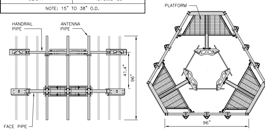
ANTENNA PLATFORM DETAIL
