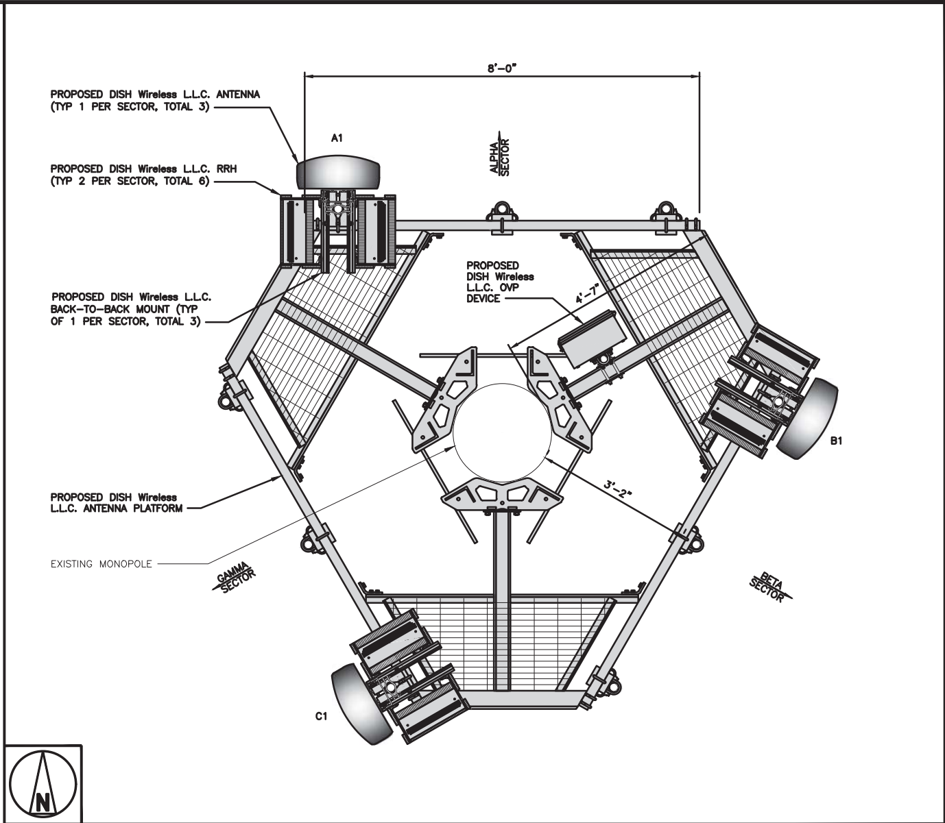
ANTENNA LAYOUT
