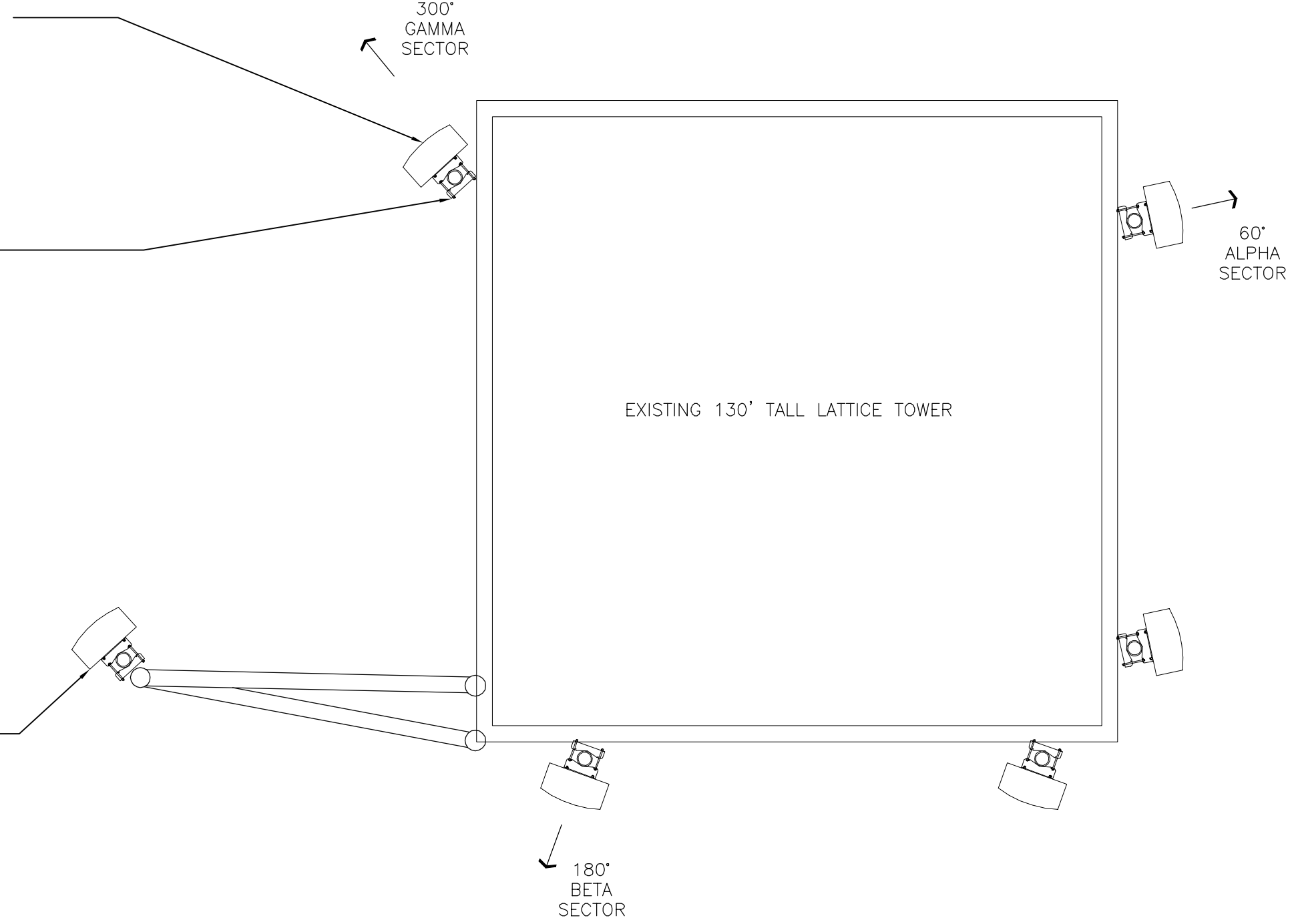
1 C-3 EXISTING ANTENNA MOUNTING CONFIGURATION SCALE: 1/2" = 1' 97' ELEVATION APPROXIMATE NORTH
