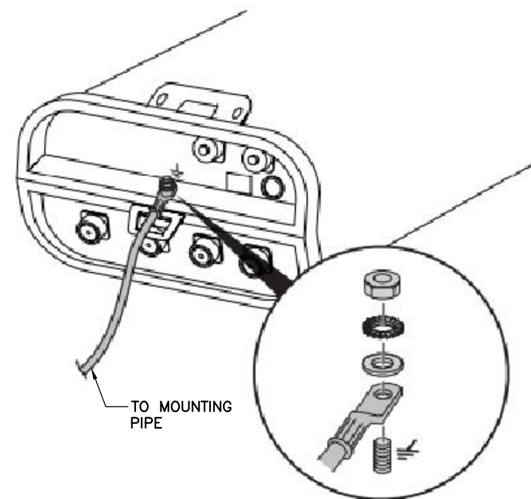
4 TYPICAL ANTENNA GROUNDING DETAIL SCALE: NONE
