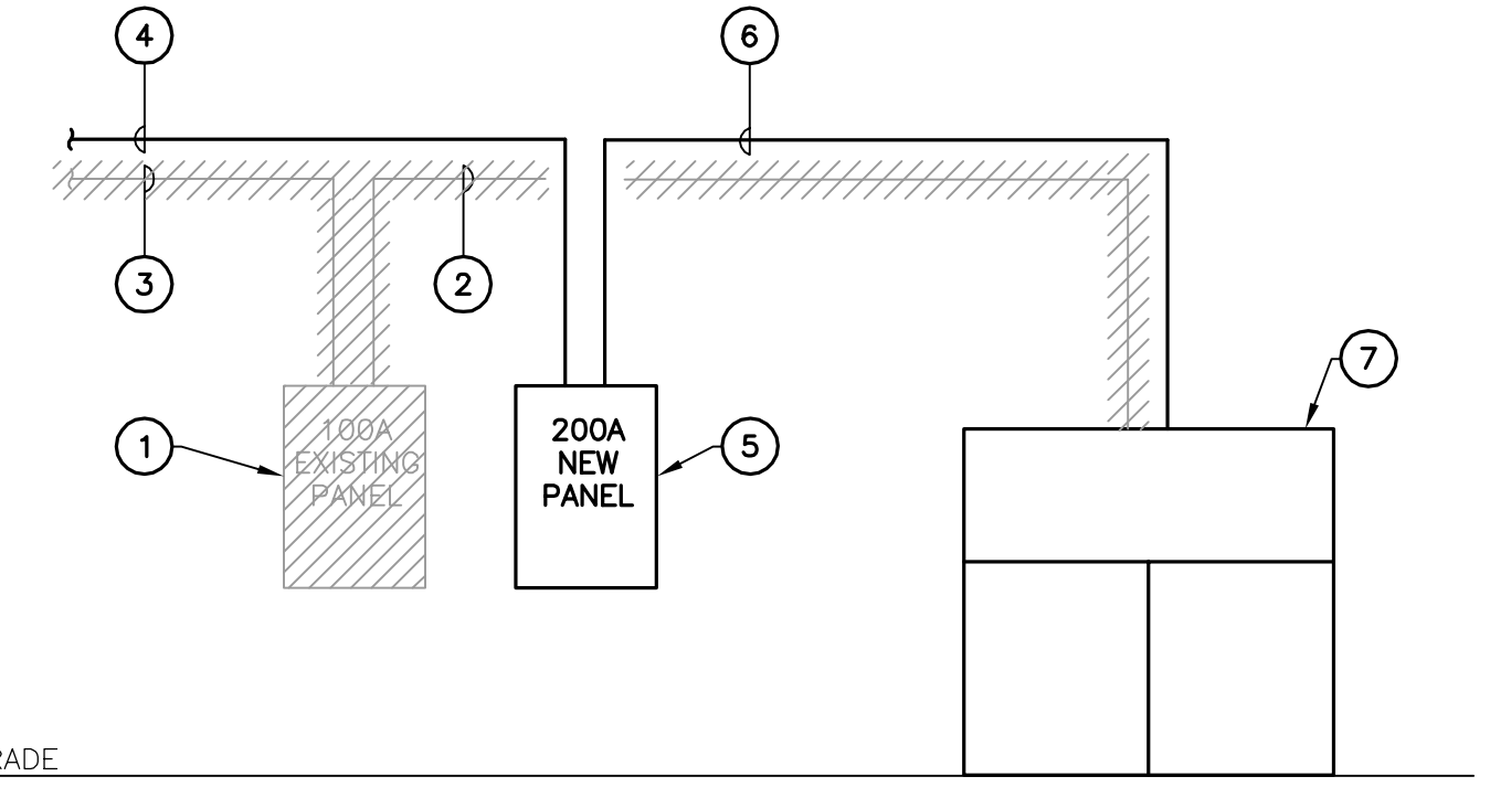
3 ELECTRICAL POWER RISER DIAGRAM E-2 NOT TO SCALE
