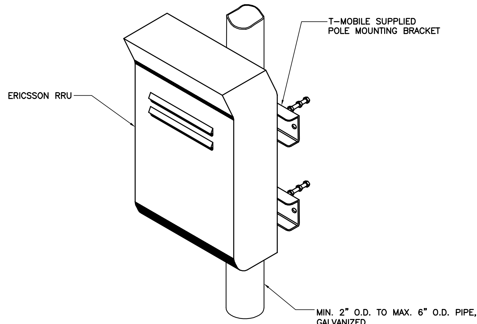
2 TYPICAL RRUS MOUNTING DETAILS E-2 SCALE: NOT TO SCALE
