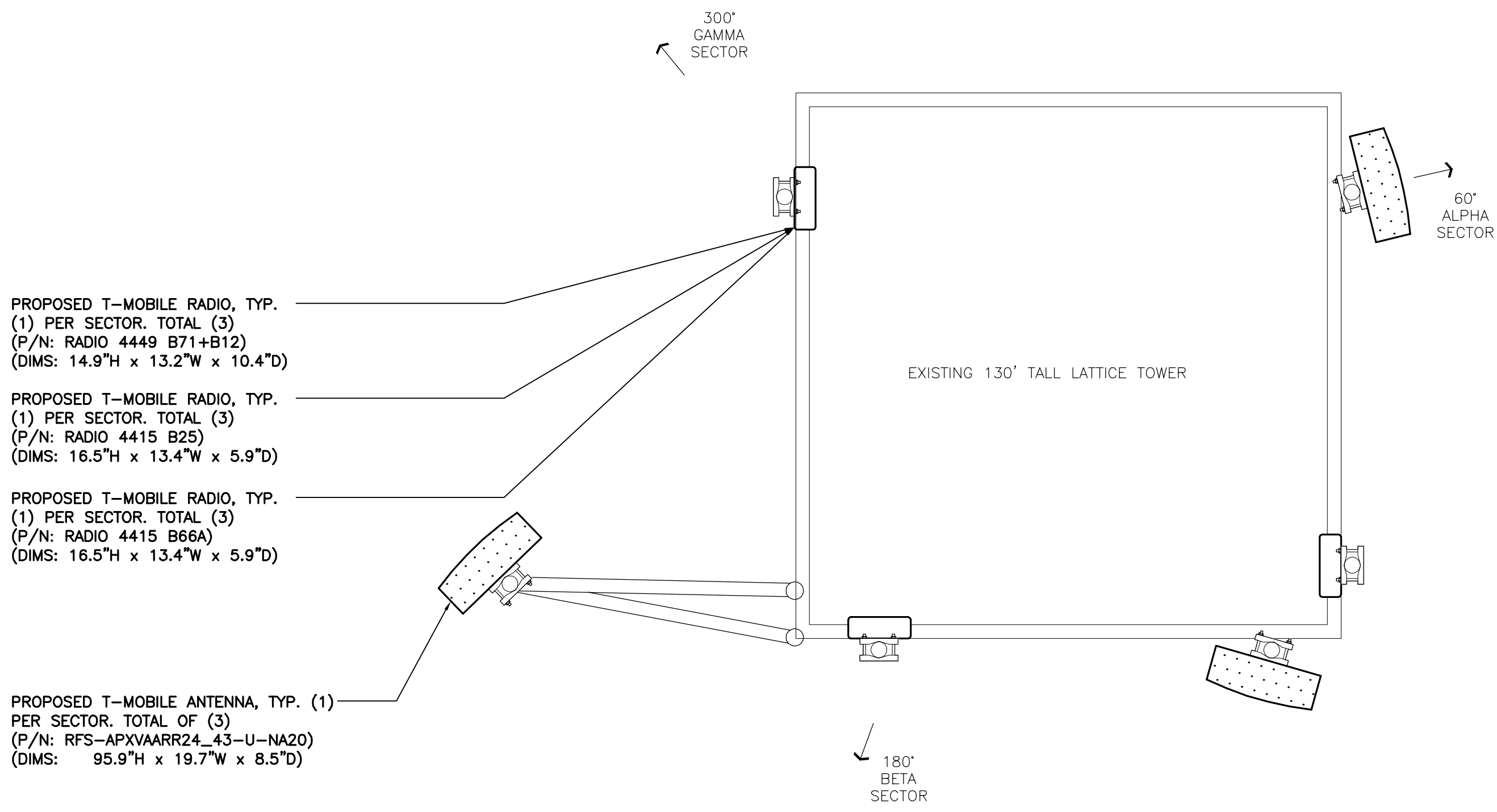
2 C-3 PROPOSED ANTENNA MOUNTING CONFIGURATION SCALE: 1/2" = 1' 97' ELEVATION APPROXIMATE NORTH
