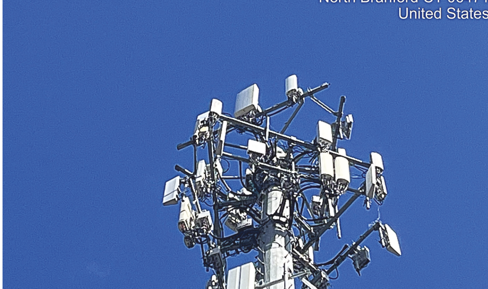
Beta sector antennas installed on existing sector frame
