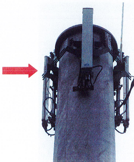
AT&T ARRAY TO BE REMOVED, SHOWN AT 47.5'
