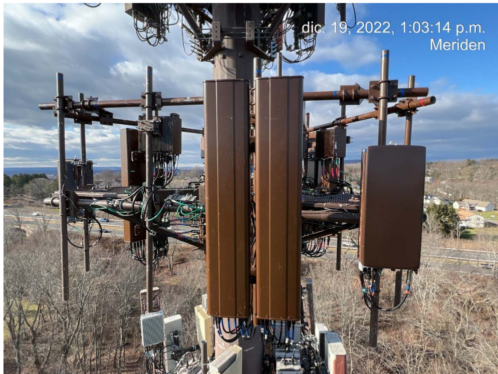
Fig. 4: Mount Modifications
