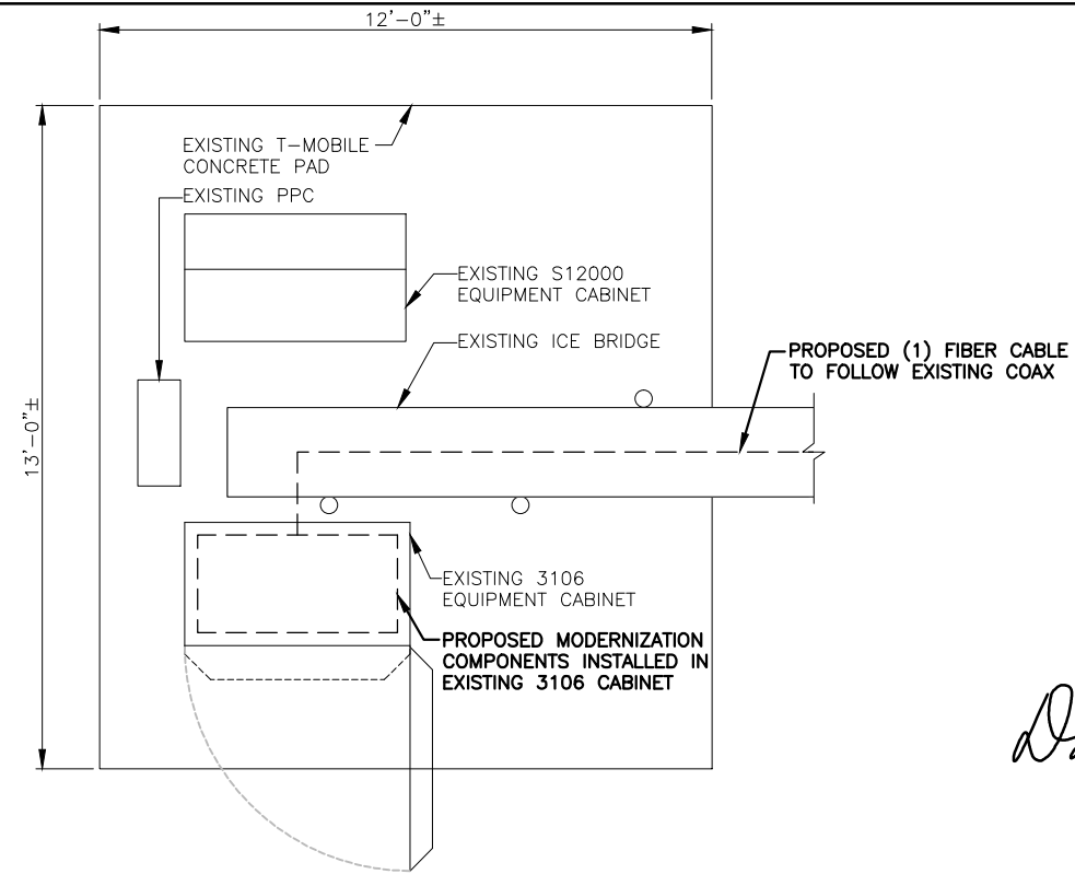
2 PROPOSED EQUIPMENT PLAN A-2 SCALE: 1/2"=1'-0" 0 1'-0" 2'-0" 4'-0" 6'-0"
