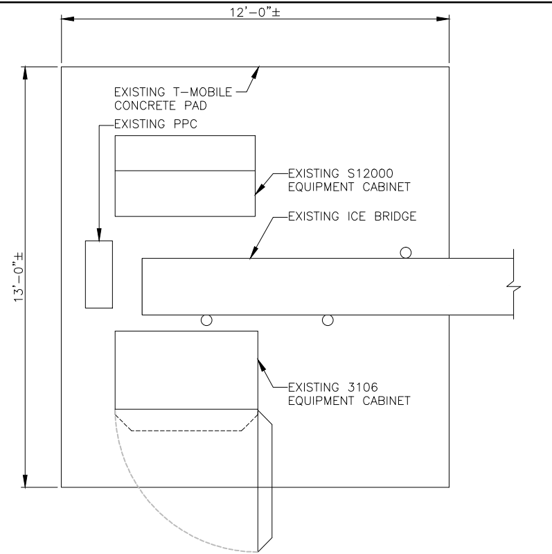
1 EXISTING EQUIPMENT PLAN A-2 SCALE: 1/2"=1'-0" 0 1'-0" 2'-0" 4'-0" 6'-0"
