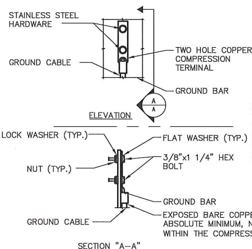
2 GROUNTING BAR CONN. DETAIL
