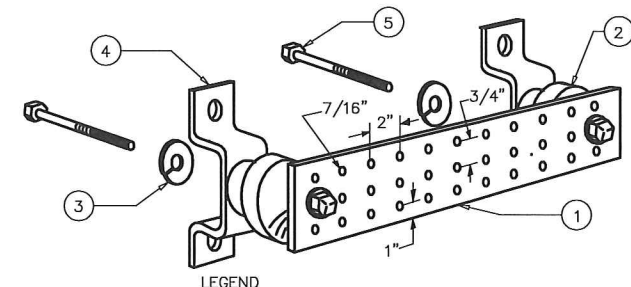
2 GROUNTING BAR CONN. DETAIL
