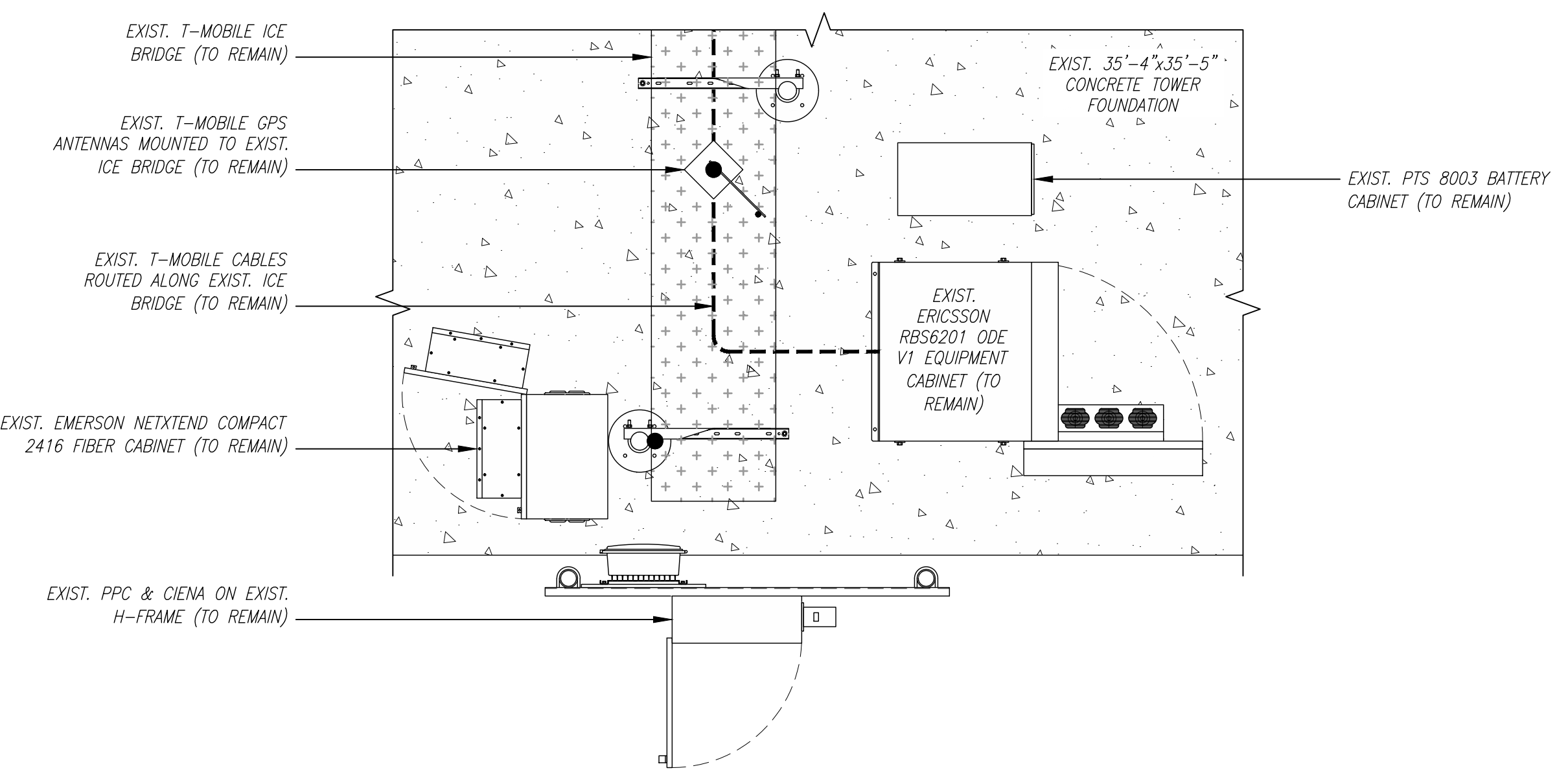
EXISTING EQUIPMENT PLAN SCALE: 1/2" = 1'-0"
