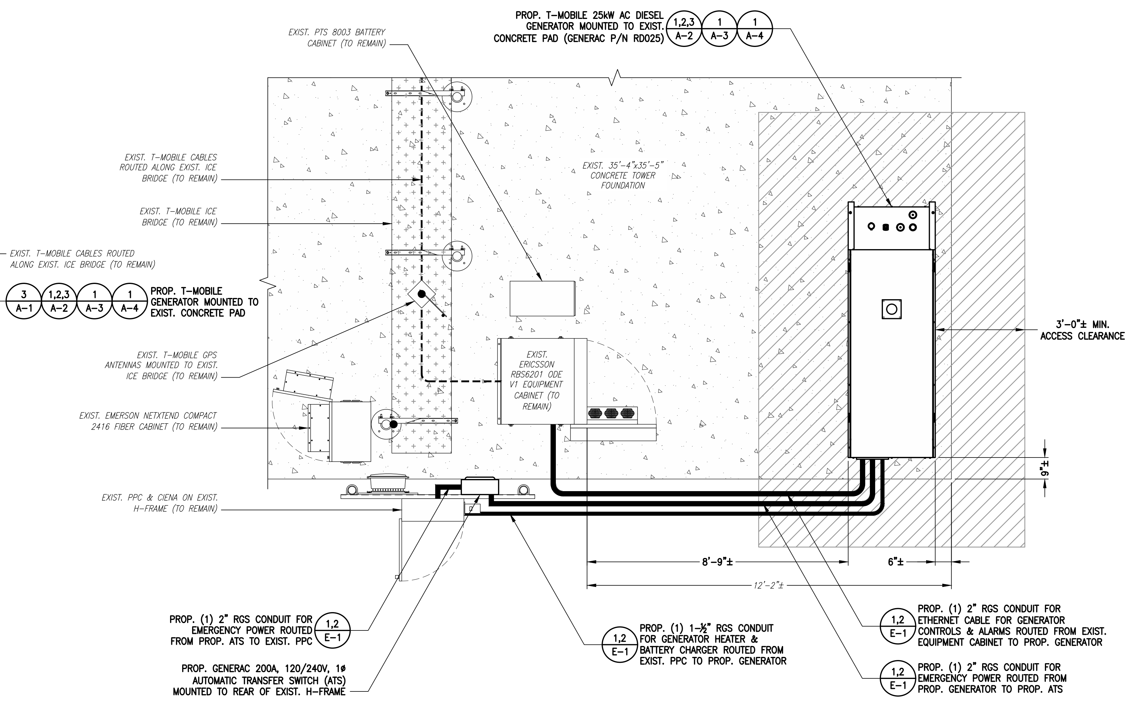
PROPOSED EQUIPMENT PLAN SCALE: 1/2" = 1'-0"
