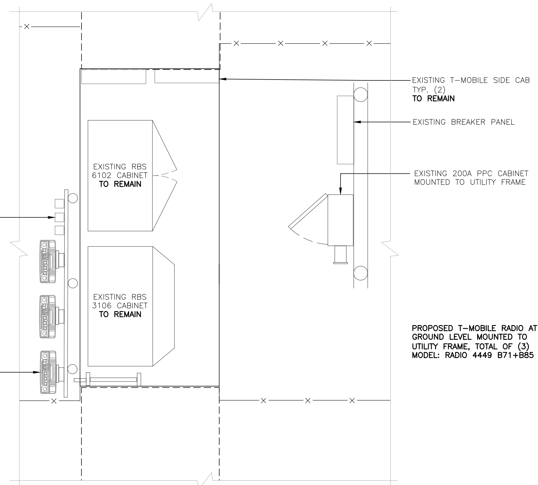
3 EQUIPMENT PLAN - EXISTING C-2 SCALE: 1/2" = 1' TRUE NORTH
