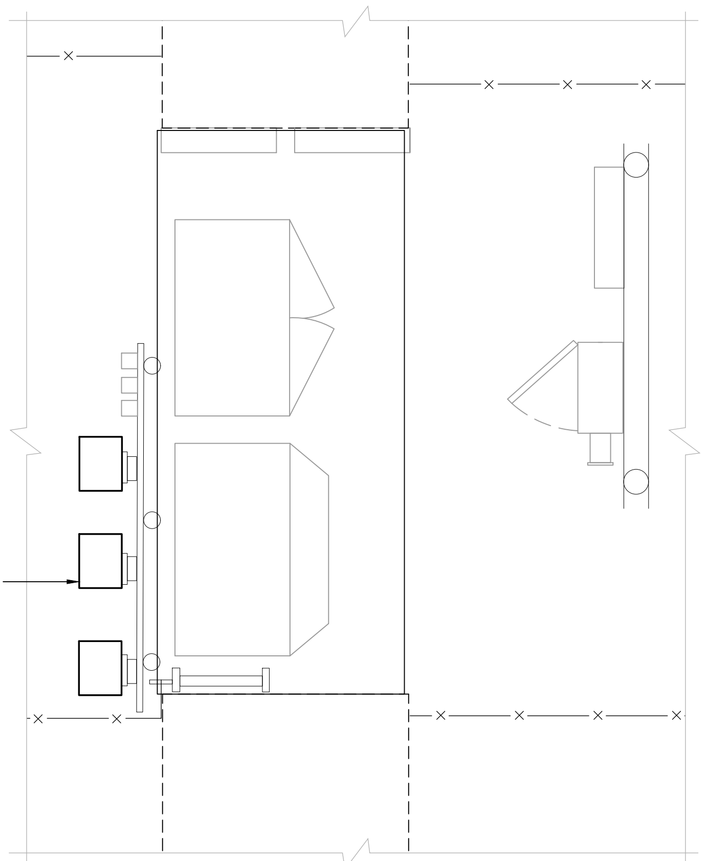
4 EQUIPMENT PLAN - PROPOSED C-2 SCALE: 3/8" = 1' TRUE NORTH
