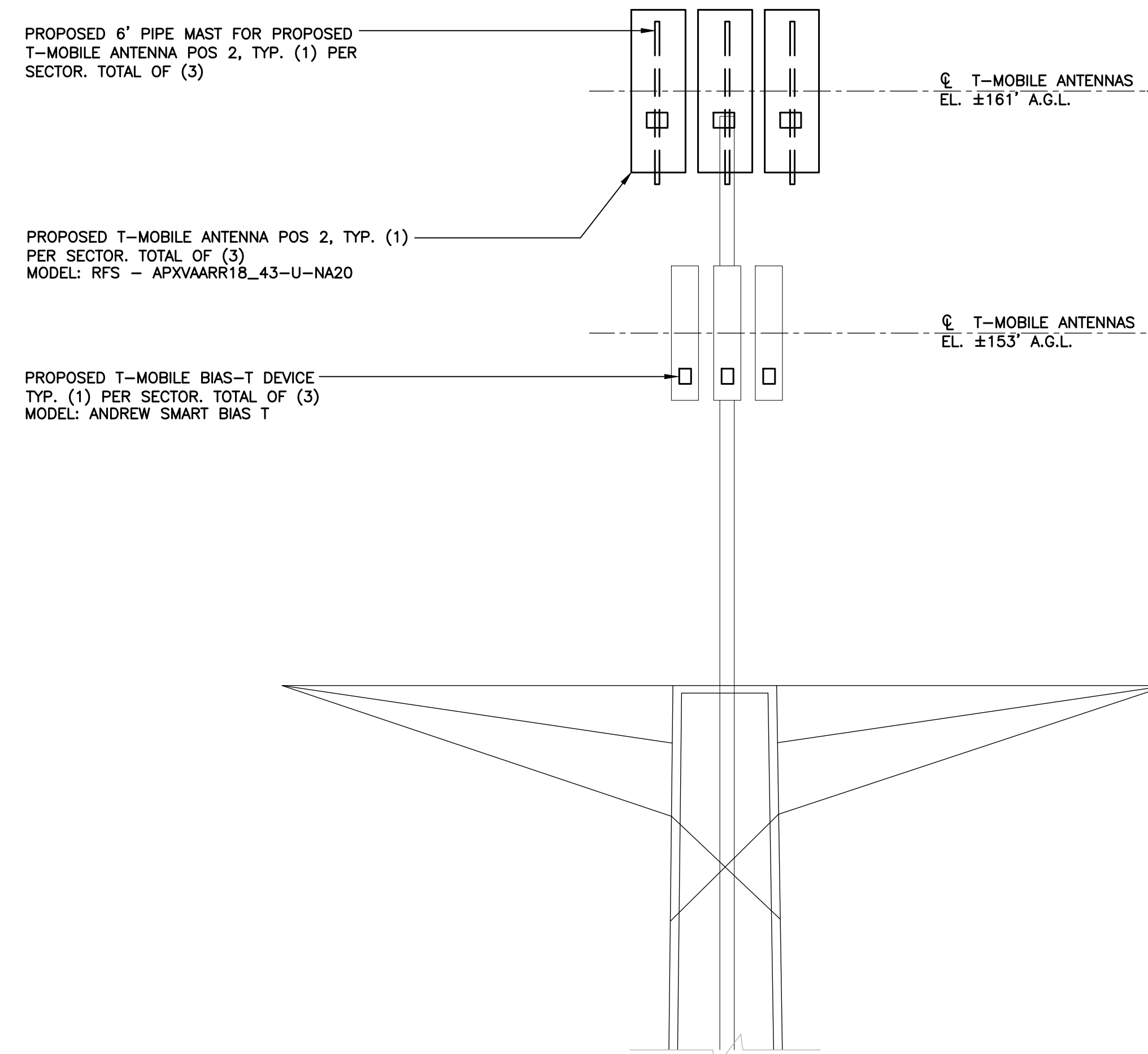
2A PROPOSED ANTENNA ELEVATION C-3 SCALE: 1/4" = 1'
