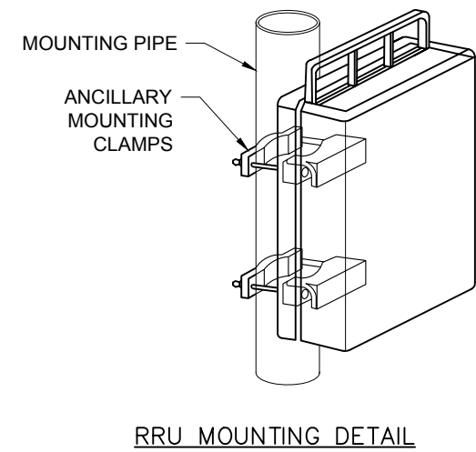
REMOTE RADIO UNIT MOUNTING DETAIL N.T.S
