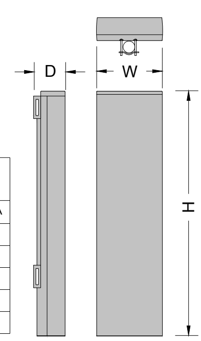
L600 ANTENNA AND RRU MOUNTING DETAIL N.T.S
