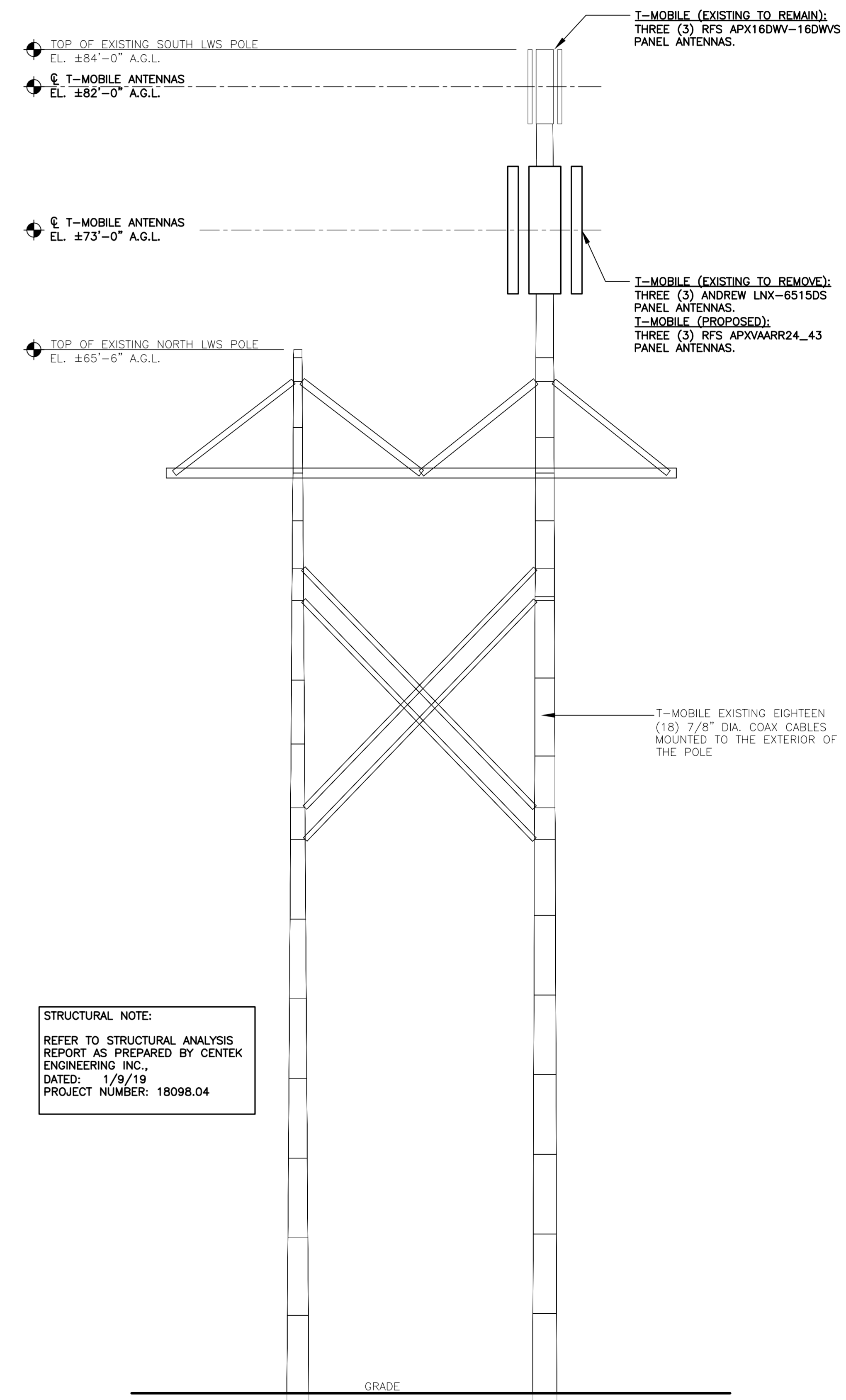
2 TOWER ELEVATION C-2 SCALE: 1" = 5' APPROX. NORTH GRAPHIC SCALE (IN FEET) 1 inch = 5 ft.
