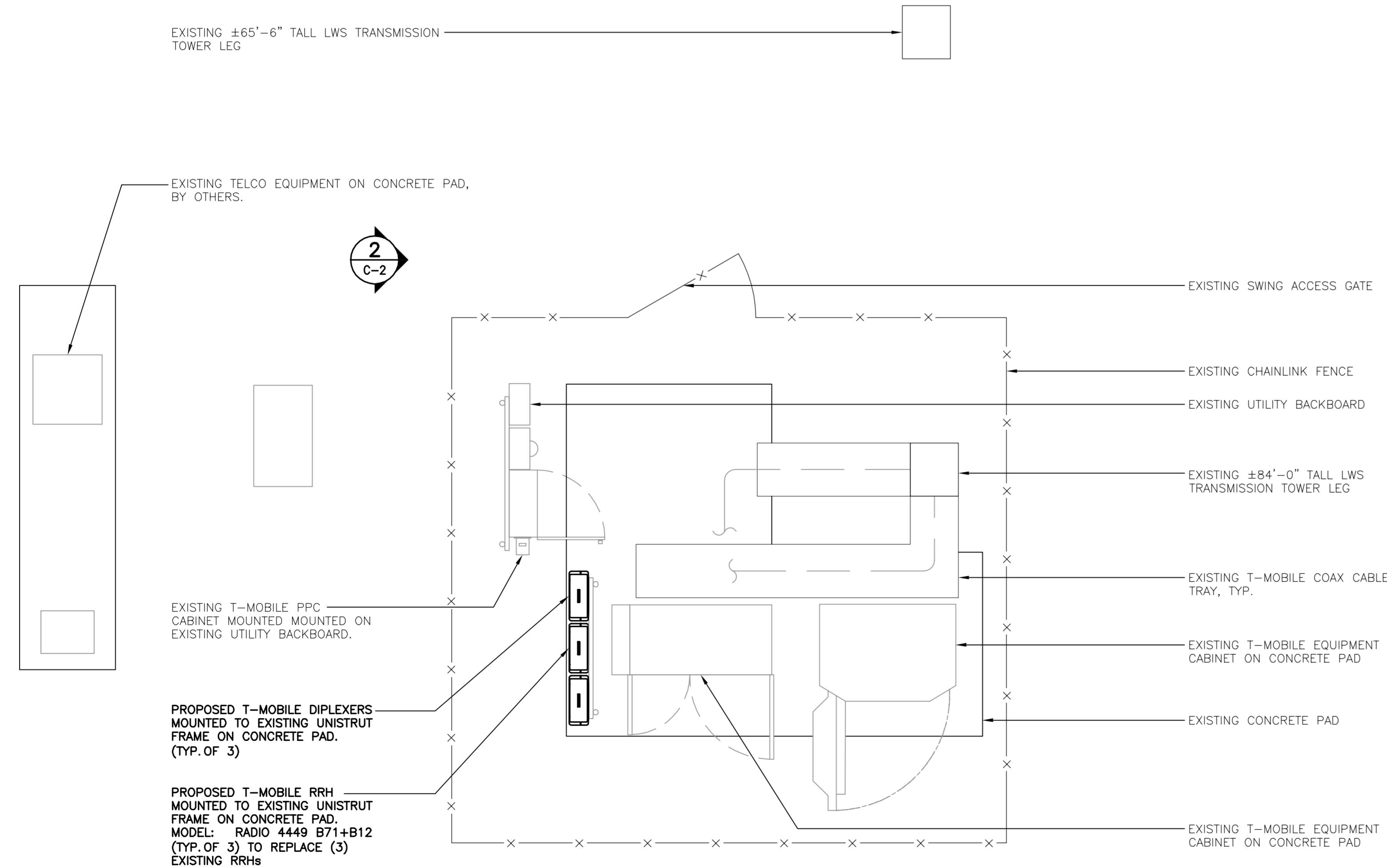
1 COMPOUND PLAN C-2 SCALE: 3/8" = 1' APPROX. NORTH GRAPHIC SCALE (IN FEET) 1 inch = 4 ft.
