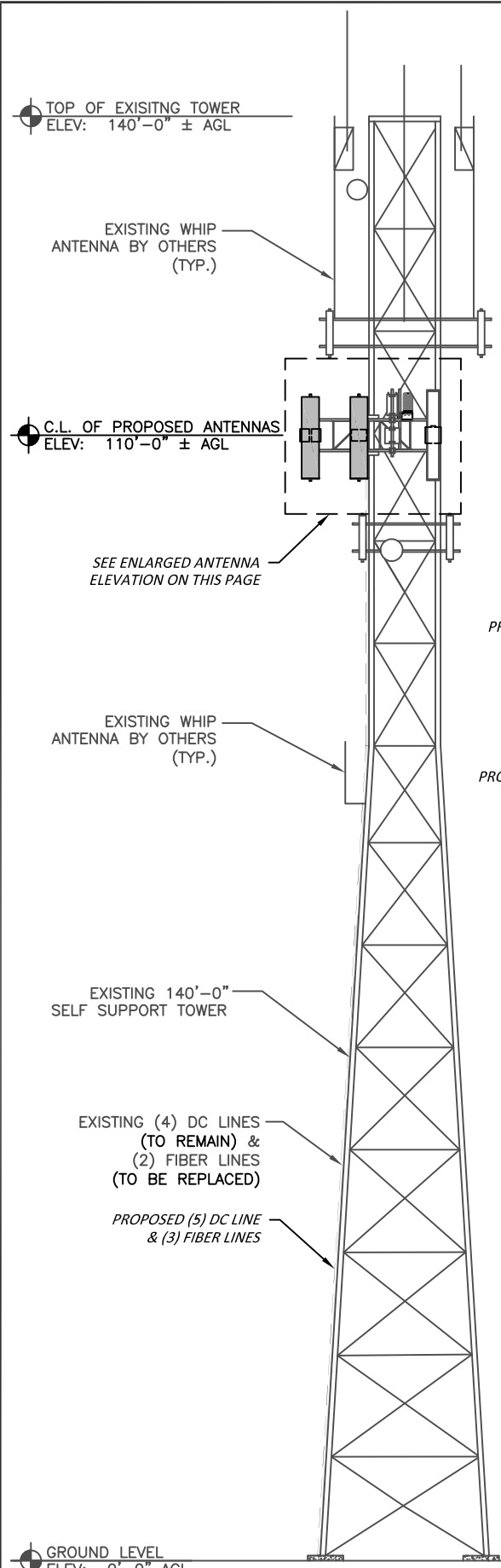
TOWER ELEVATION SCALE: 1/4" = 1'-0" (22"X34") 1/8" = 1'-0" (11"X17")
