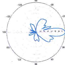
0° | Vertical | 750 MHz
