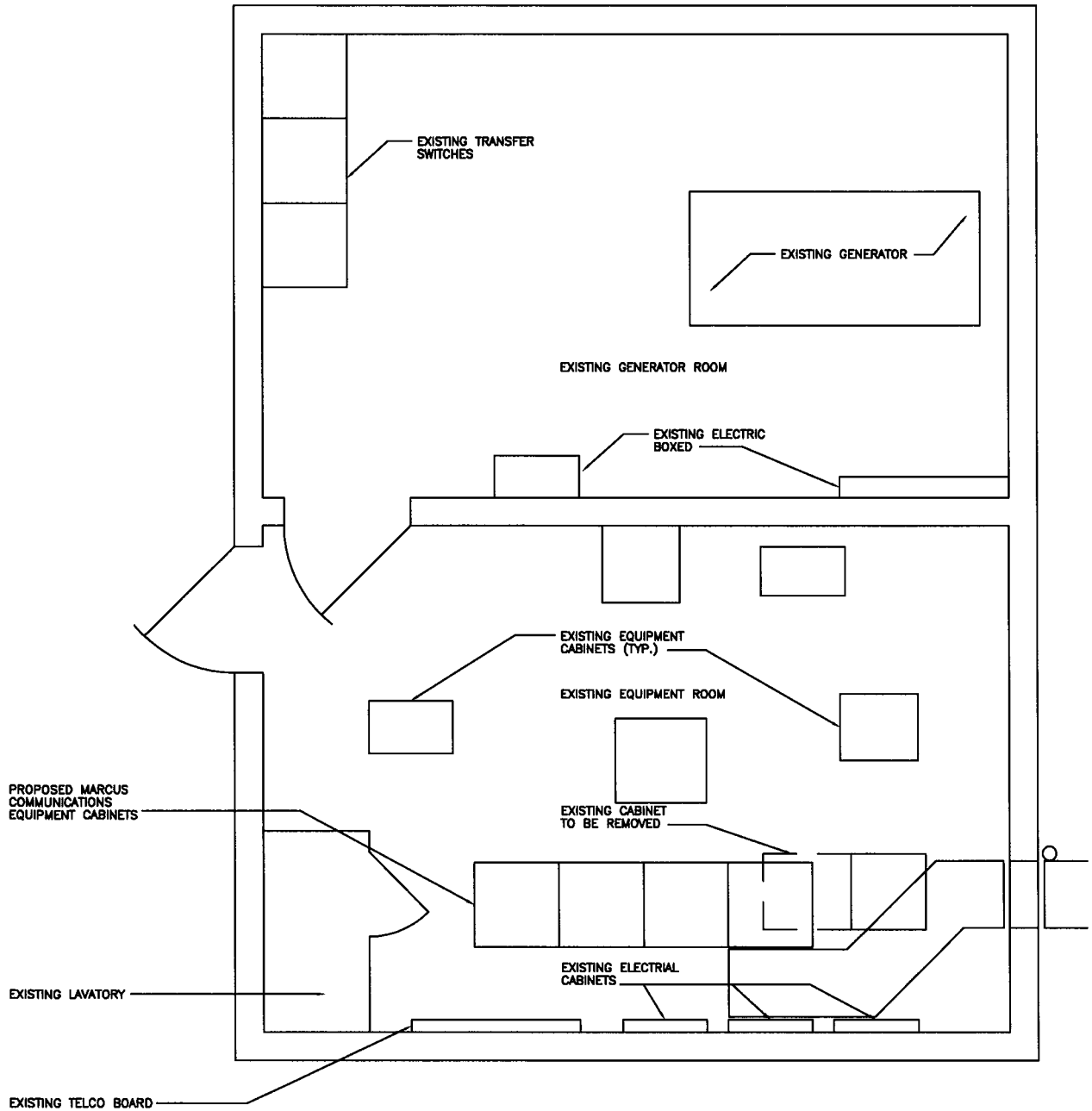
1 EQUIPMENT ROOM PLAN L-2 SCALE: 1/4" = 1'-0"
