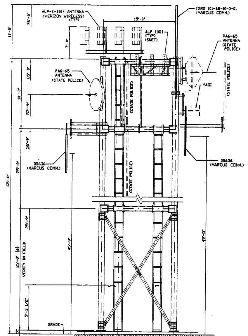
TOWER ELEVATION FACE A SCALE: 3/16"=1'-0"
