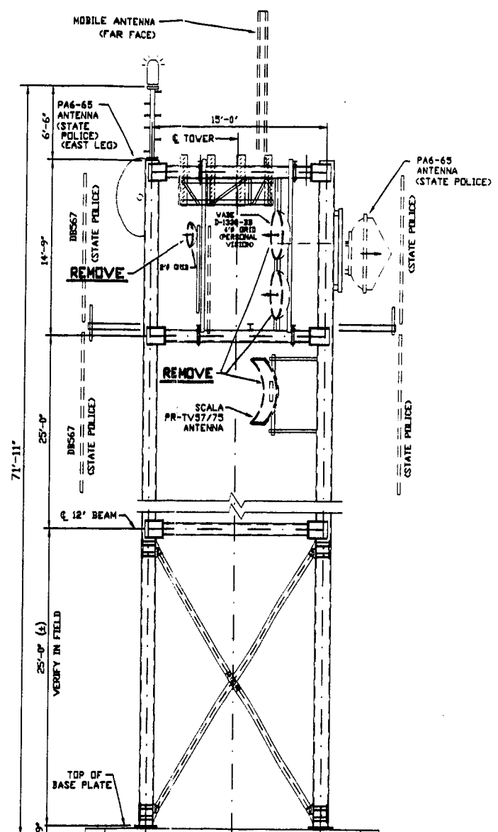
TOWER ELEVATION FACE C SCALE: 3/16"=1'-0"
