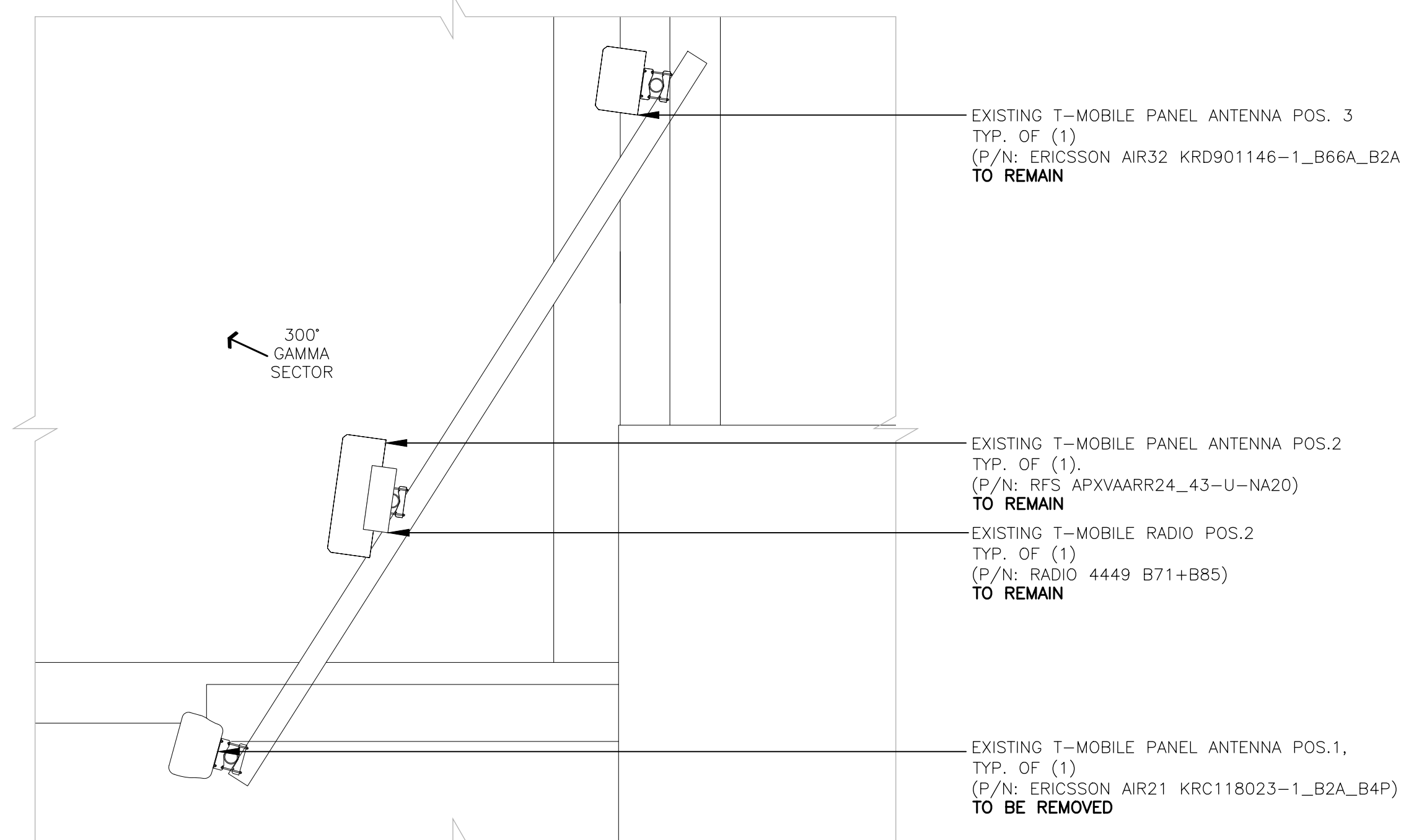
3 EXISTING ANTENNA PLAN (GAMMA) C-3 SCALE: 1/2" = 1' TRUE NORTH
