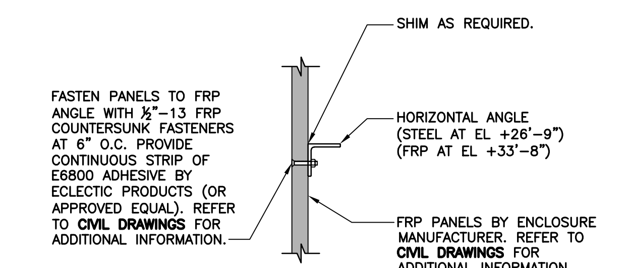
9 TYPICAL PANEL TO ANGLE CONNECTION S-1 SCALE: 1" = 1'-0"
