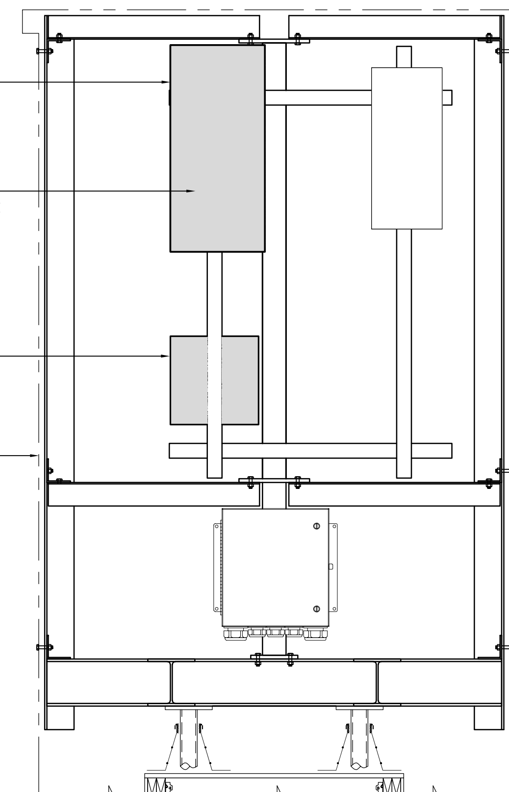
2 PROPOSED ANTENNA CONFIGURATION PLAN SCALE: 1" = 1'-0" NORTH
