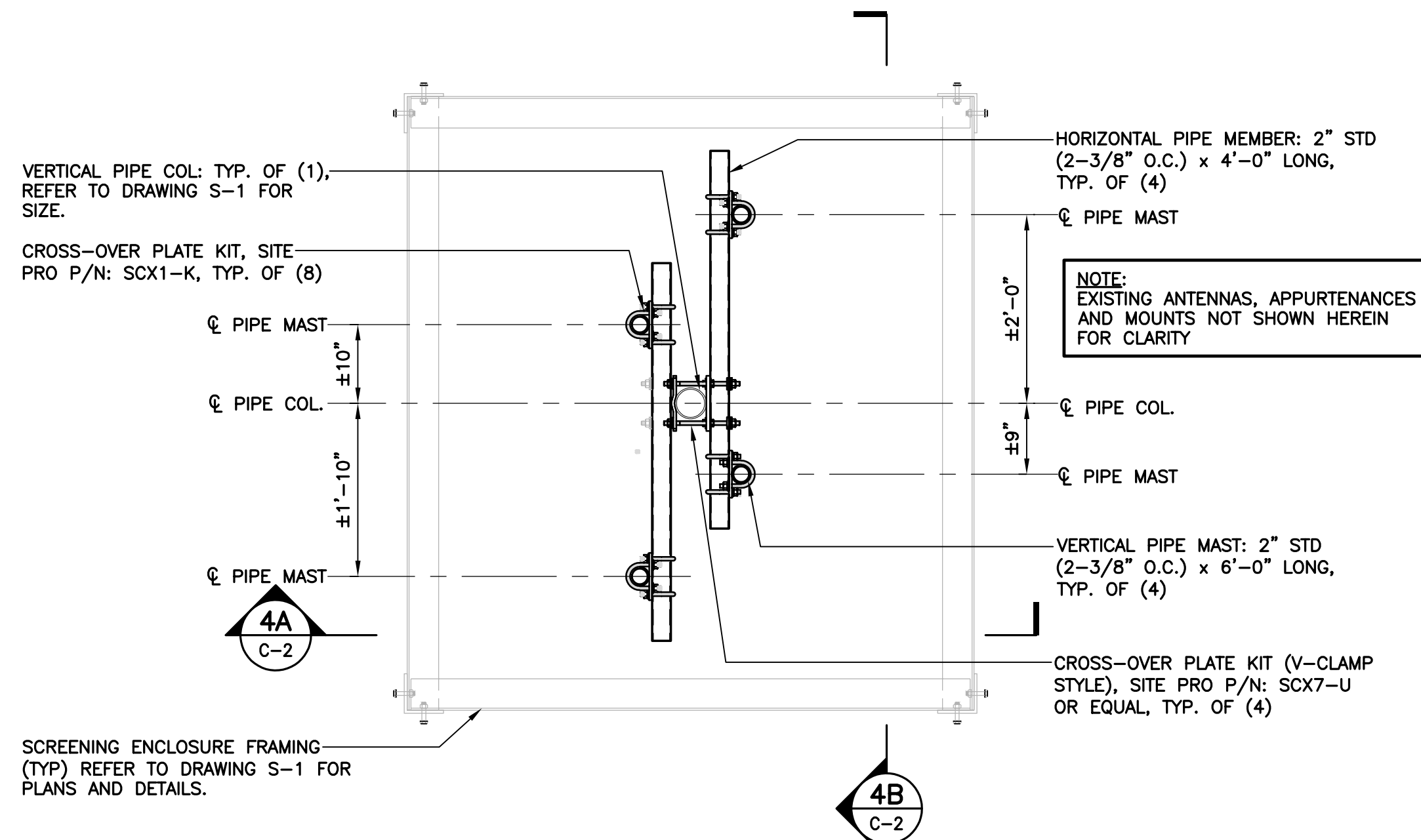
4 ANTENNA MOUNT ASSEMBLY PLAN SCALE: 3/4" = 1'-0" NORTH
