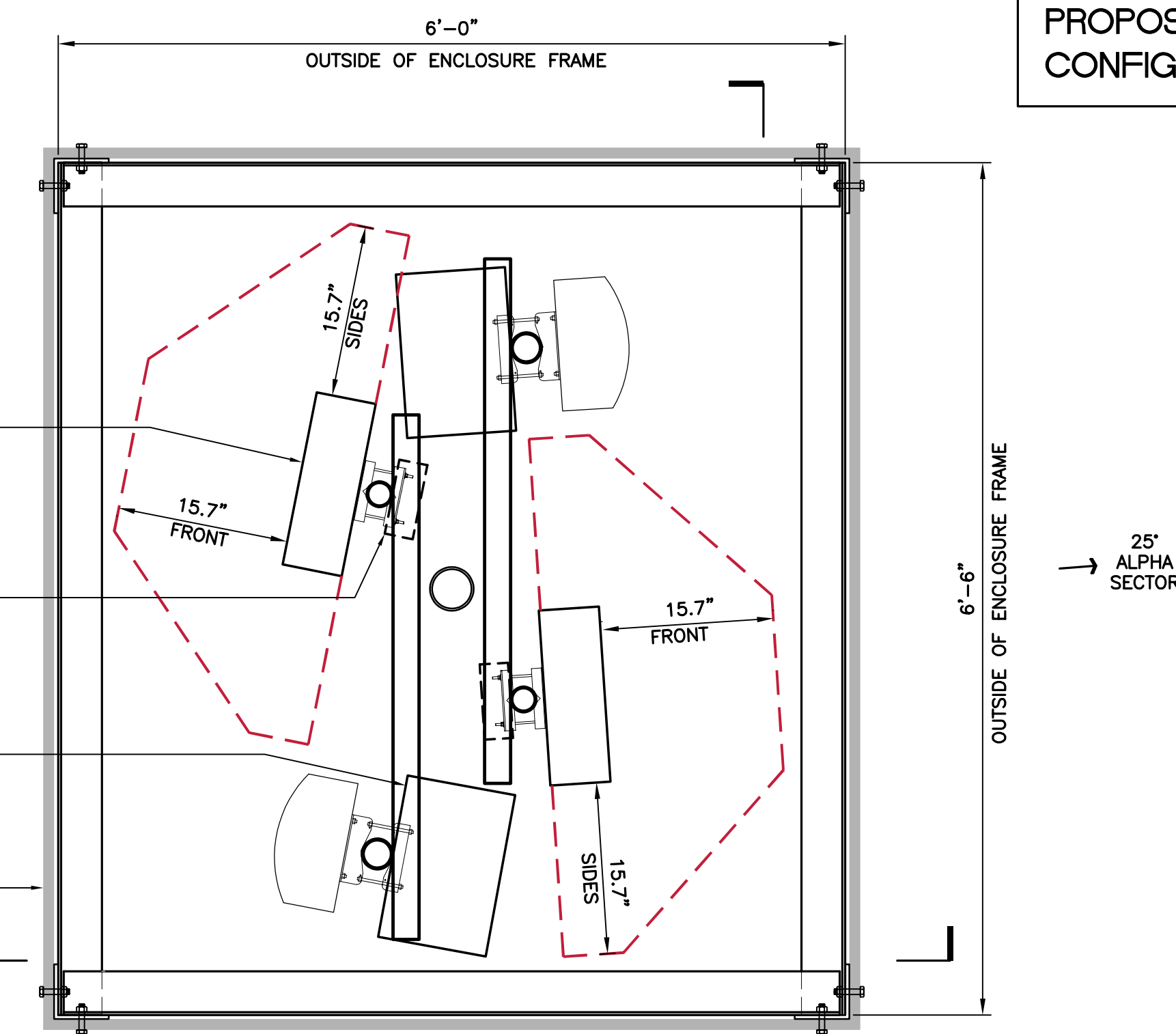
2 PROPOSED ANTENNA CONFIGURATION PLAN SCALE: 1" = 1'-0" NORTH
