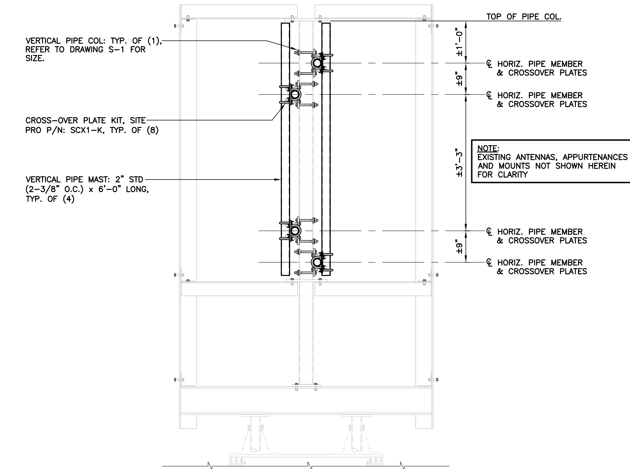
4A ANTENNA MOUNT ASSEMBLY SECTION SCALE: 3/4" = 1'-0"
