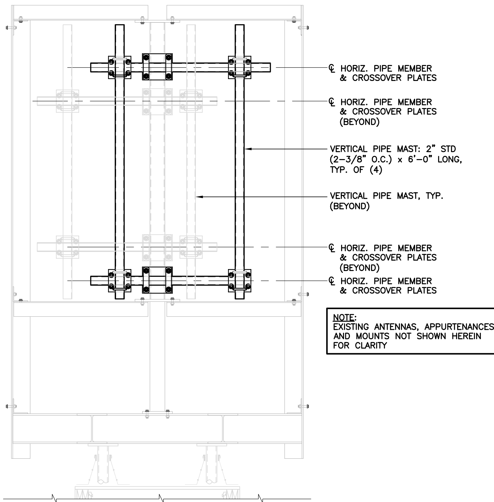
4B ANTENNA MOUNT ASSEMBLY SECTION SCALE: 3/4" = 1'-0"
