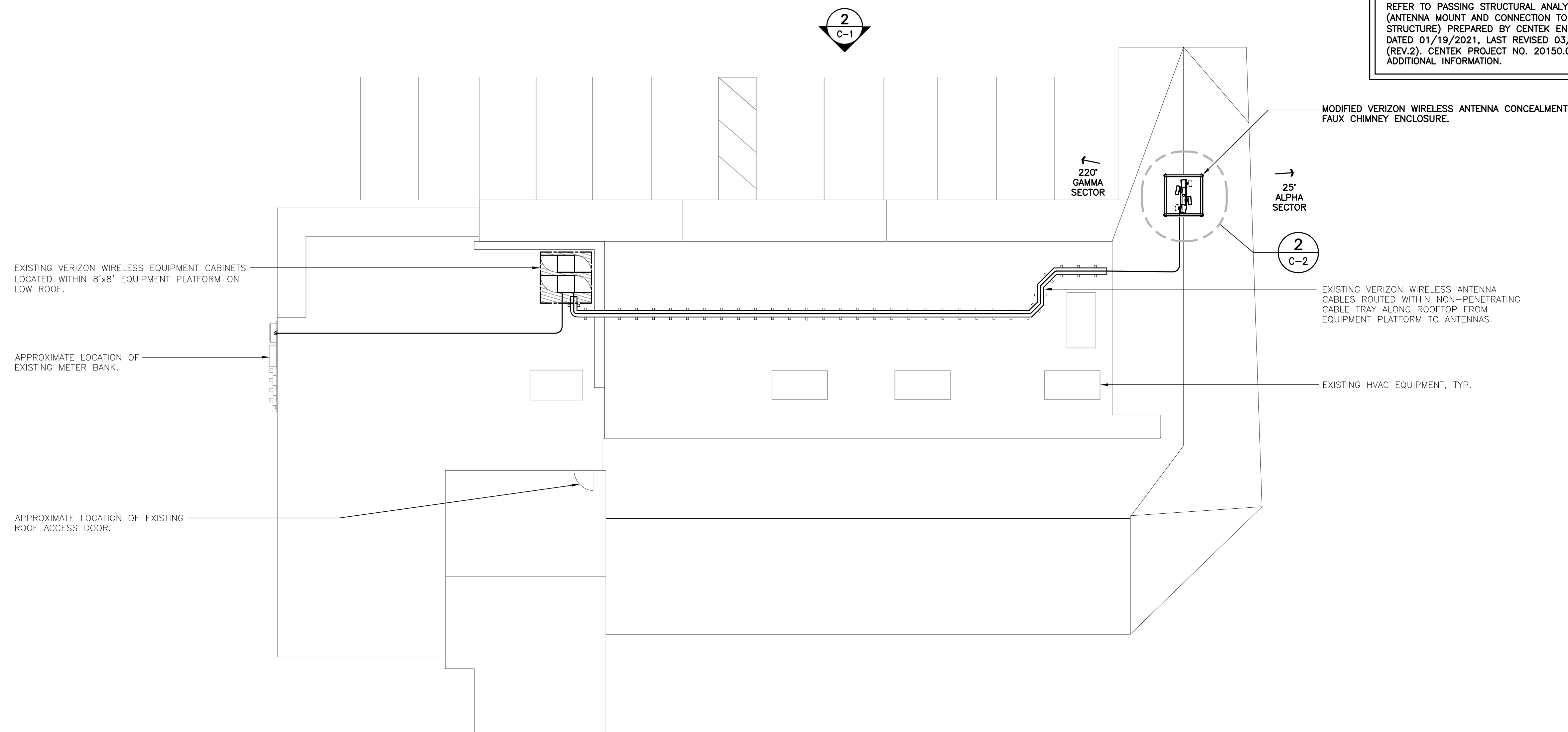
1 PARTIAL SITE/ROOF PLAN - PROPOSED CONDITIONS SCALE: 1" = 10'
