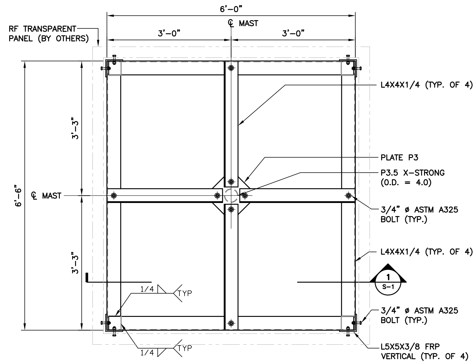
4 PLAN - HIGH FRAMING S-1 SCALE: 3/4" = 1'-0"
