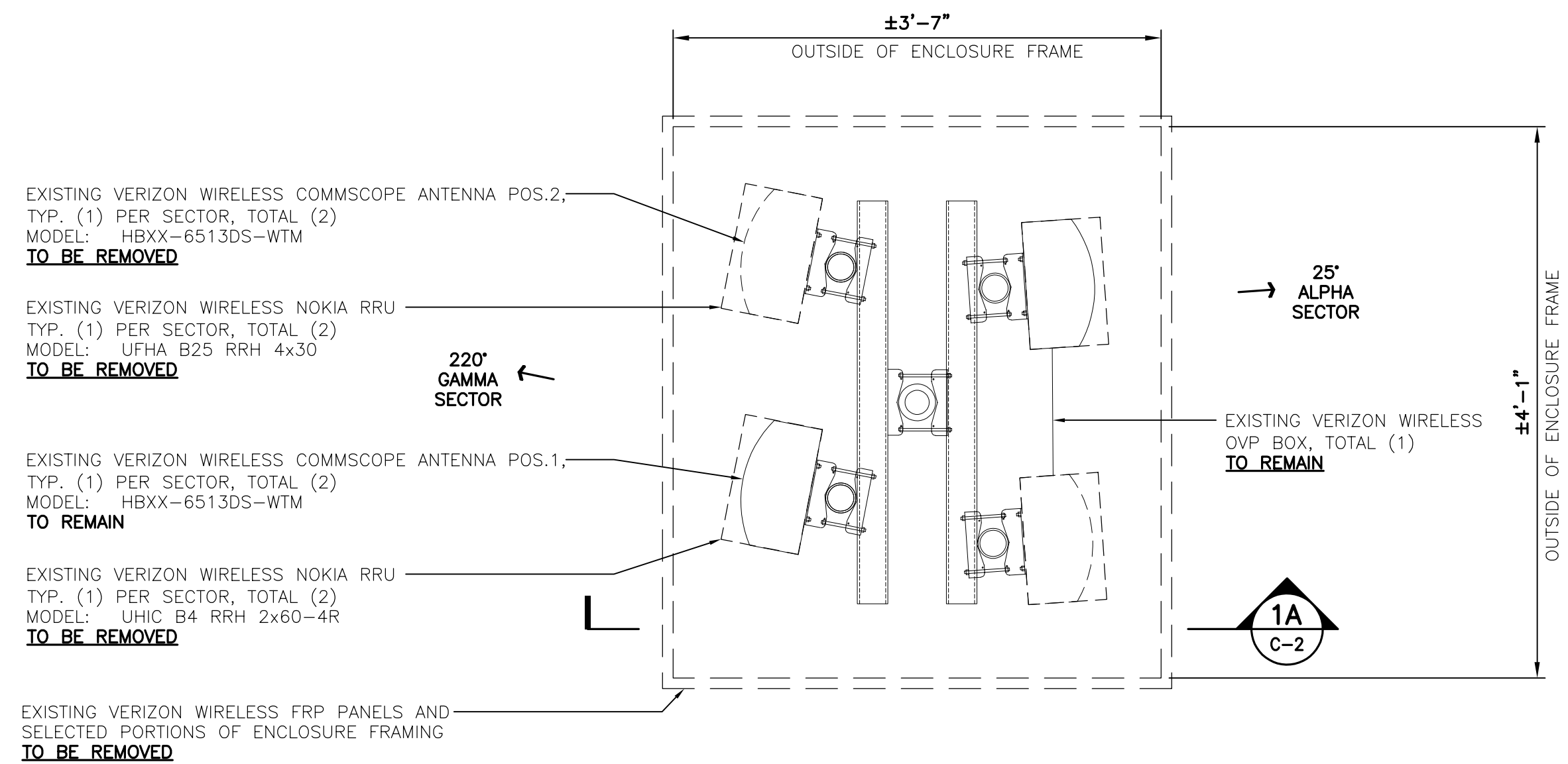
1 EXISTING ANTENNA CONFIGURATION PLAN SCALE: 1" = 1'-0" NORTH
