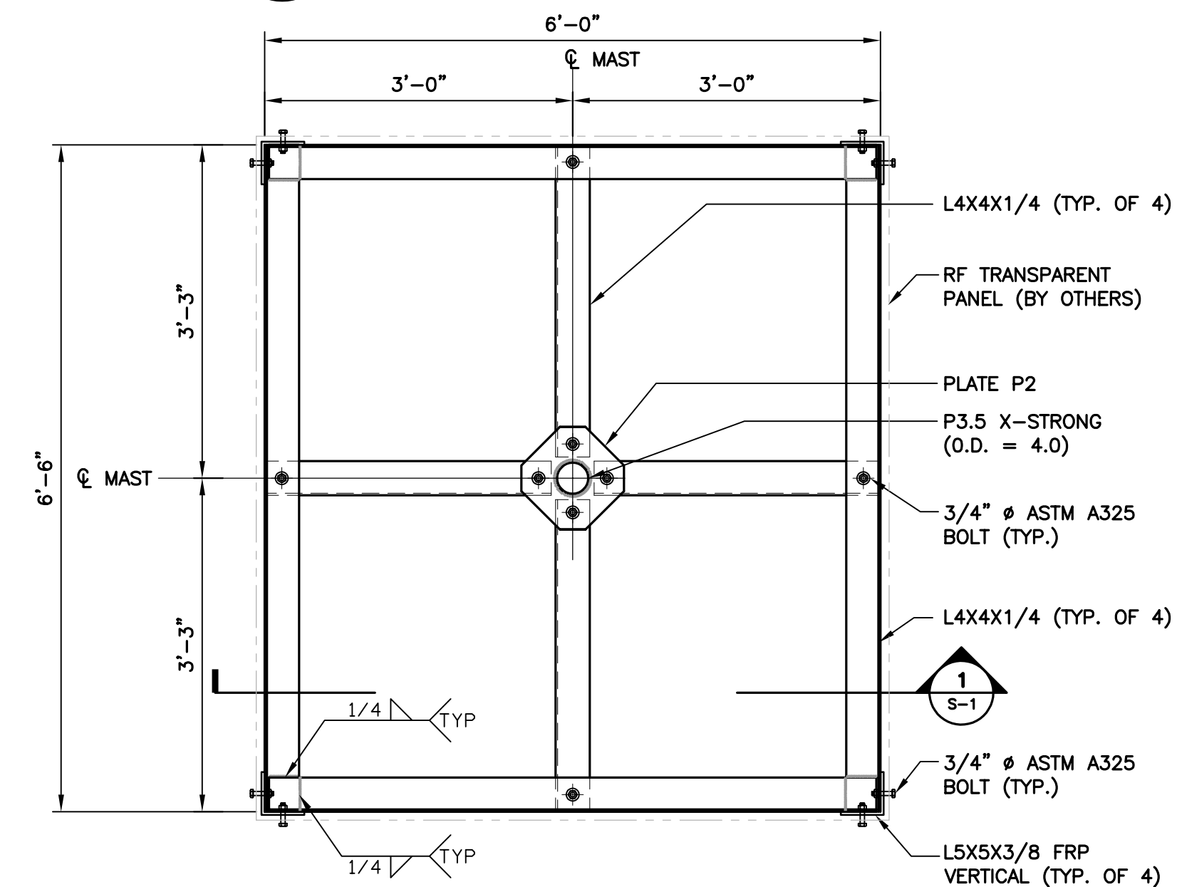
3 PLAN - MID FRAMING S-1 SCALE: 3/4" = 1'-0"
