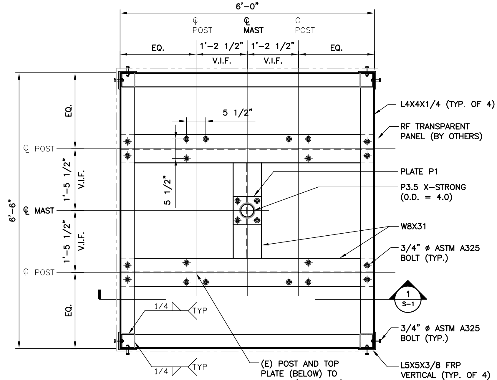
2 PLAN - LOW FRAMING S-1 SCALE: 3/4" = 1'-0"
