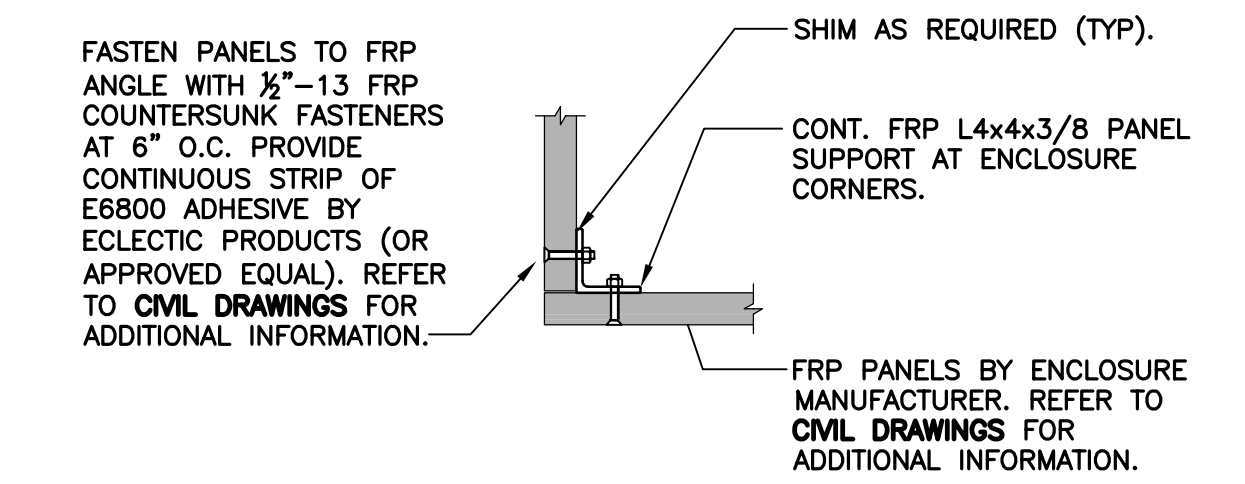
8 PLAN - TYPICAL FRP CORNER CONNECTION S-1 SCALE: 1" = 1'-0"
