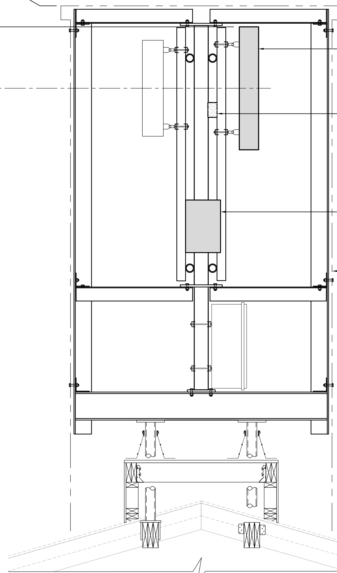
2A PROPOSED ANTENNA CONFIGURATION SECTION SCALE: 3/4" = 1'-0"
