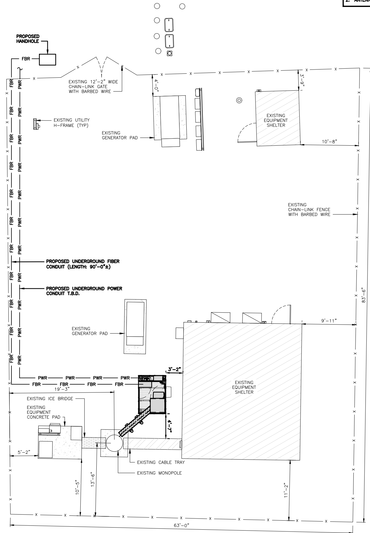
UTILITY ROUTE PLAN
