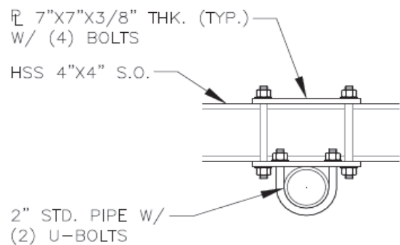
S.O. MOUNT DETAIL
