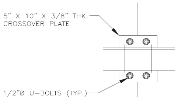
CROSSOVER PLATE DETAIL
